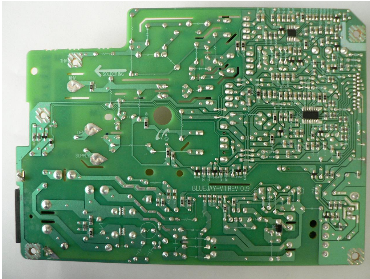
SUNGHO, Bluejay V1 SF-760P SMPS & HVPS PBA_Rear
