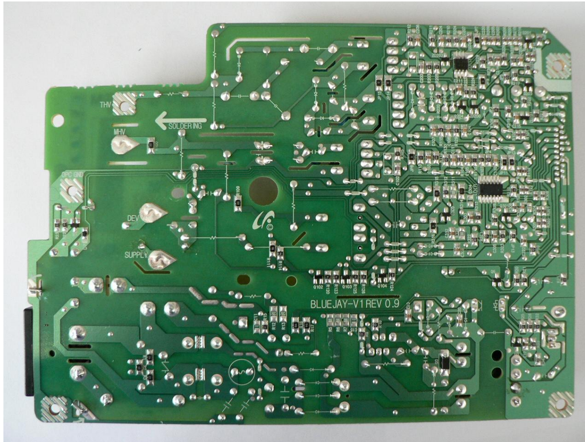
SHANDONG, Bluejay V1 SF-760P SMPS & HVPS PBA_Rear
