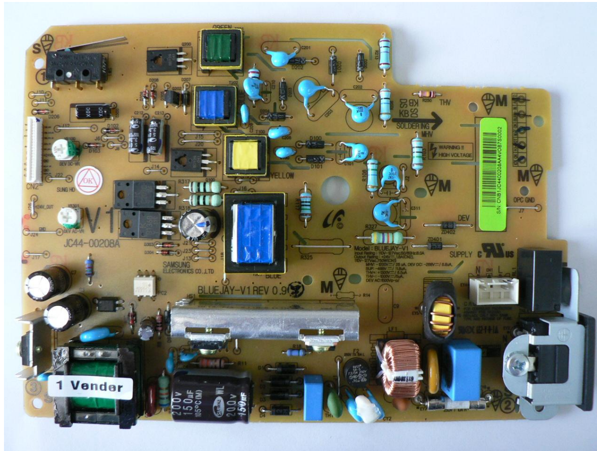
SUNGHO, Bluejay V1 SF-760P SMPS & HVPS PBA_Front
