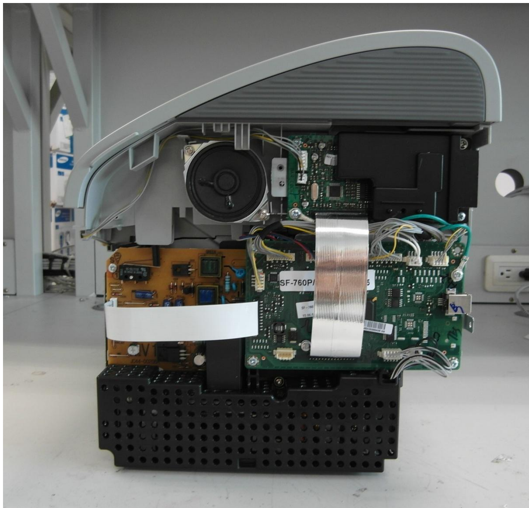
SF-760P SIDE_LEFT
