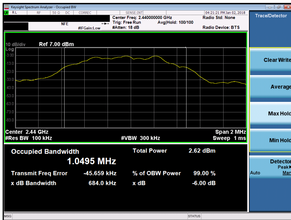
Plot 7-1. Occupied Bandwidth Plot (Bluetooth LE – Ch. 19)
