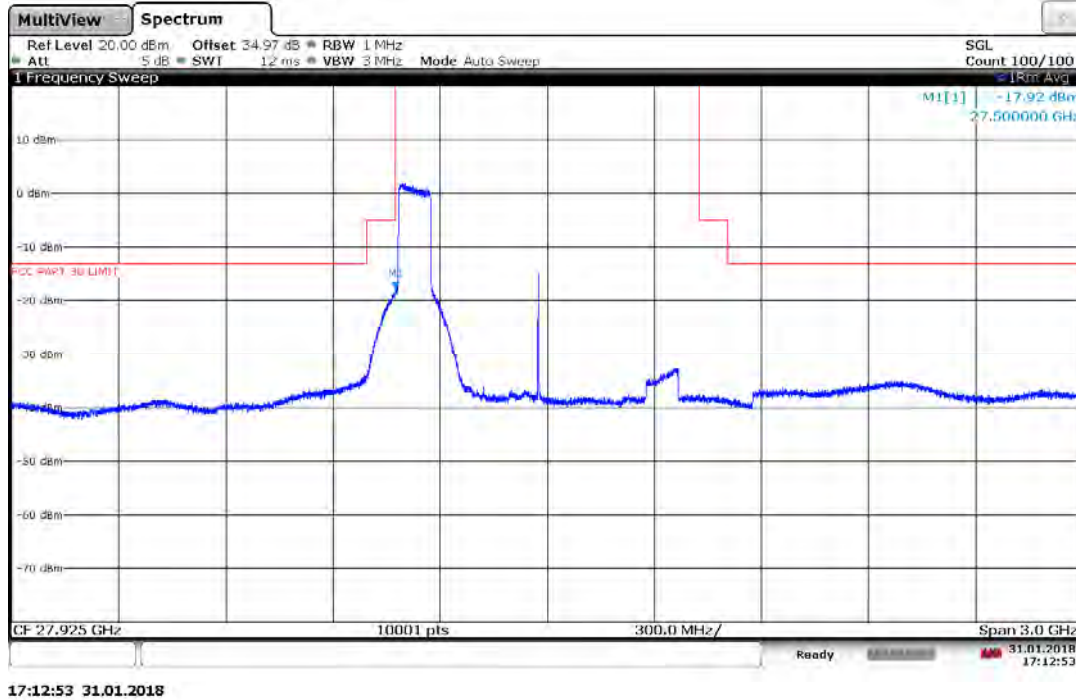
Plot 7-93. Band Edge Plot (1CC QPSK Low Channel)
