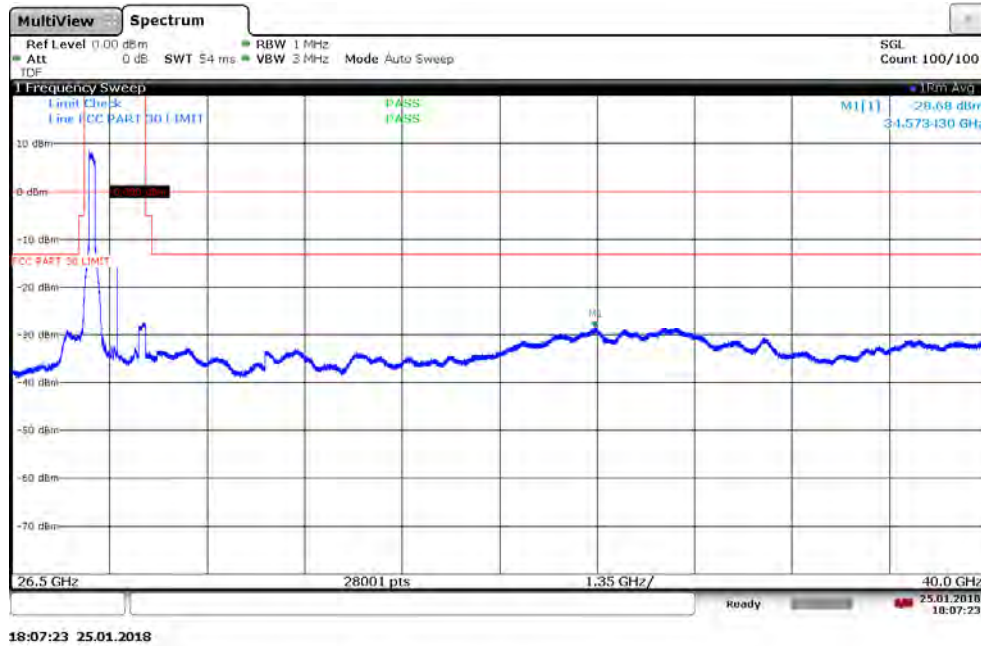
Plot 7-79. Antenna B Radiated Spurious Plot 26.5-40 GHz (1CC QPSK High Channel)
