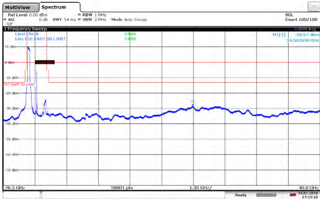
Plot 7-50. Antenna A Radiated Spurious Plot 26.5-40 GHz (1CC QPSK Mid Channel)
