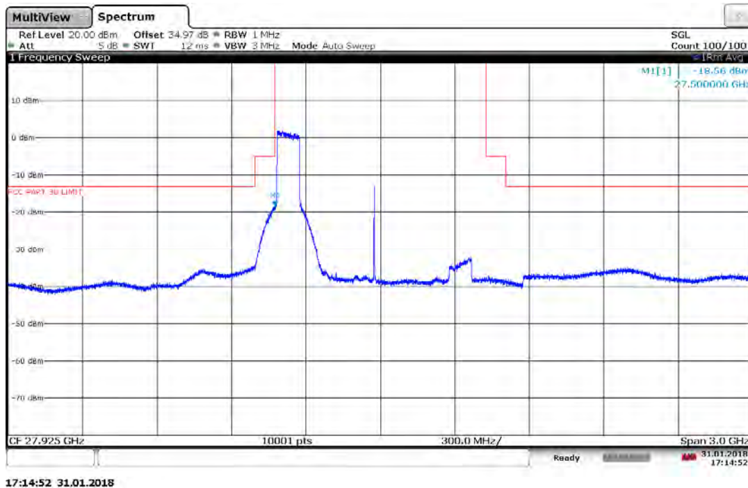
Plot 7-94. Band Edge Plot (1CC 16QAM Low Channel)
