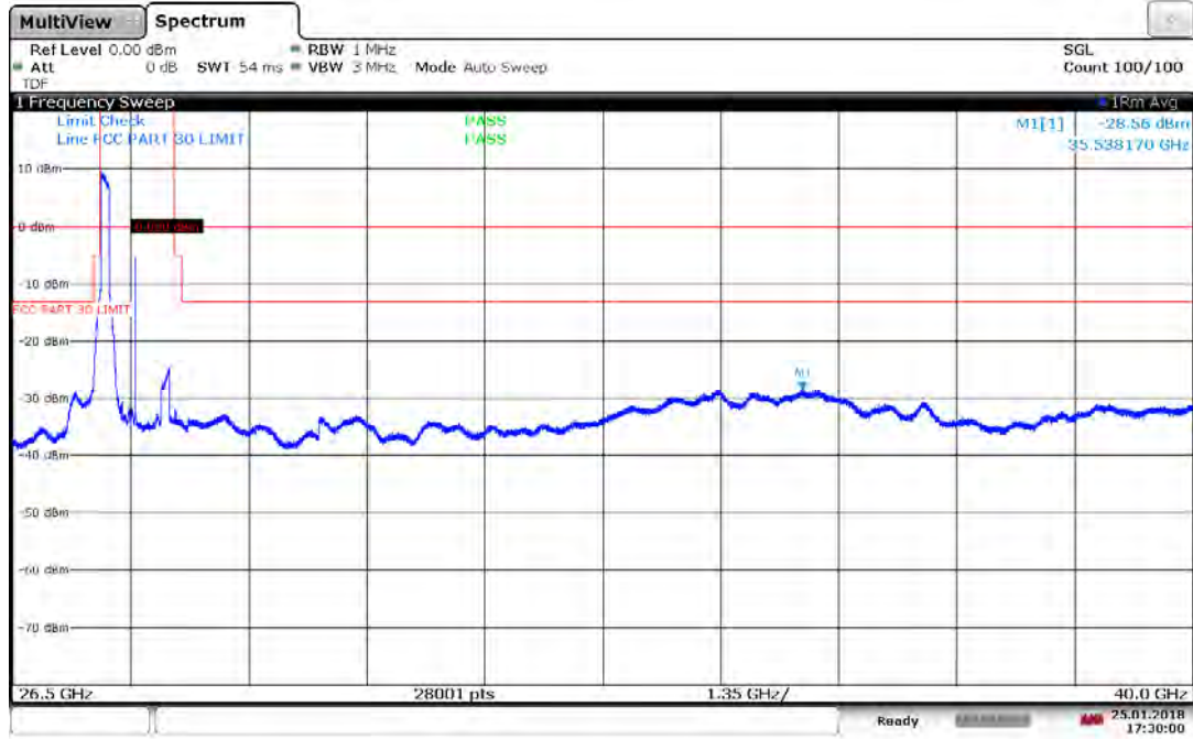
Plot 7-49. Antenna A Radiated Spurious Plot 26.5-40 GHz (1CC QPSK Low Channel)
