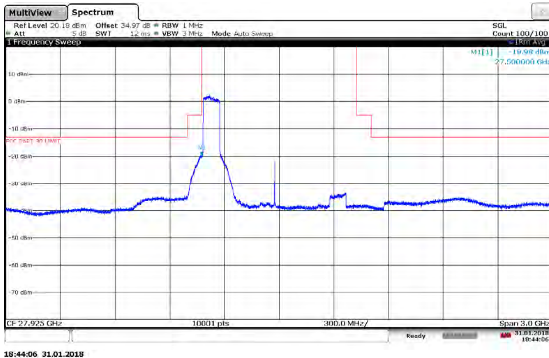
Plot 7-106. Band Edge Plot (1CC 16QAM Low Channel)
