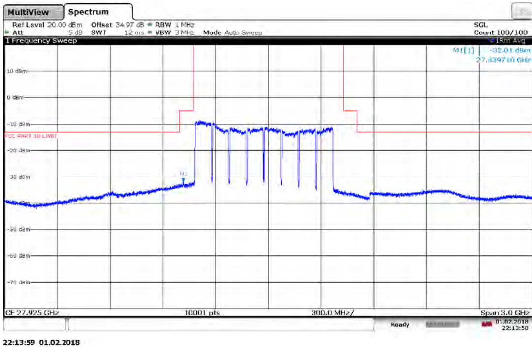
Plot 7-96. Band Edge Plot (8CC QPSK Low Channel)
