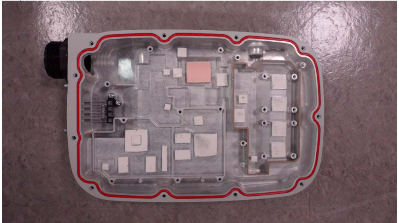
Internal Photo Without Modules
