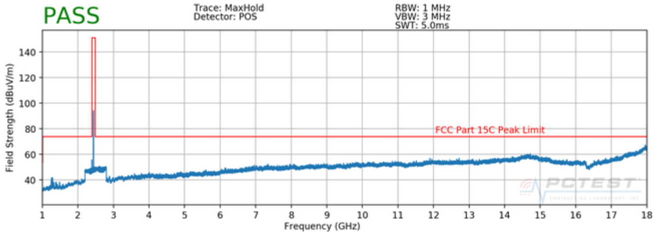
Plot 7-5. Radiated Spurious Plot above 1GHz (BTLE – Ch. 39, Ant. Pol. V)
