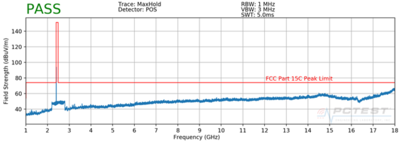
Plot 7-2. Radiated Spurious Plot above 1GHz (BTLE – Ch. 0, Ant. Pol. H)
