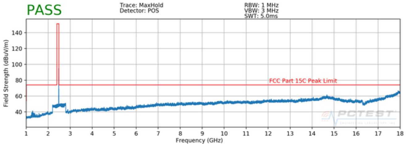
Plot 7-7. Radiated Spurious Plot above 1GHz (BTLE – Ch. 78, Ant. Pol. V)
