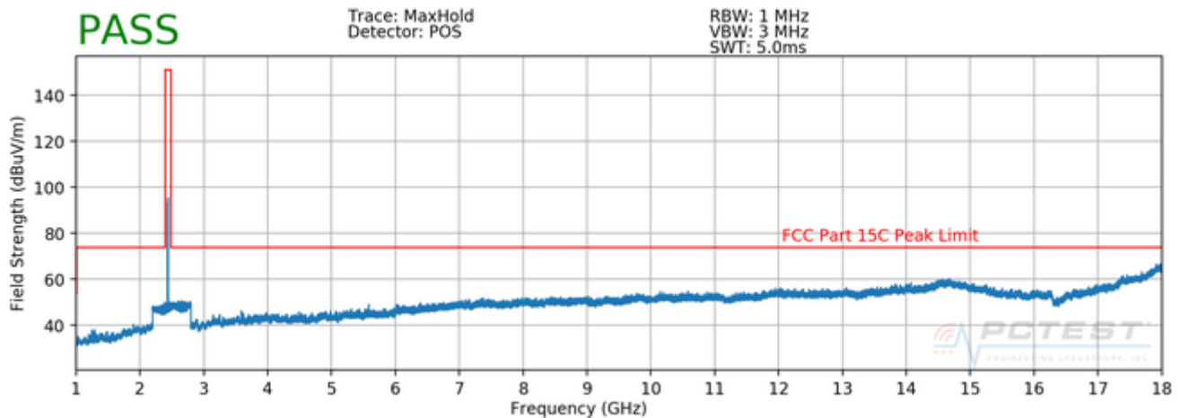
Plot 7-4. Radiated Spurious Plot above 1GHz (BTLE – Ch. 39, Ant. Pol. H)
