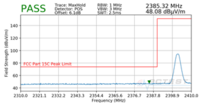
Plot 7-15. Radiated Restricted Lower Band Edge Measurement (Peak)
