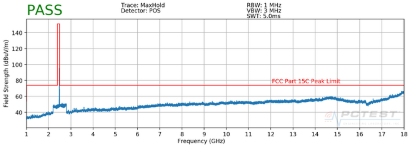
Plot 7-6. Radiated Spurious Plot above 1GHz (BTLE – Ch. 78, Ant. Pol. H)
