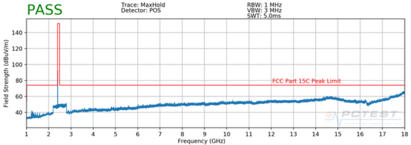
Plot 7-3. Radiated Spurious Plot above 1GHz (BTLE – Ch. 0, Ant. Pol. V)
