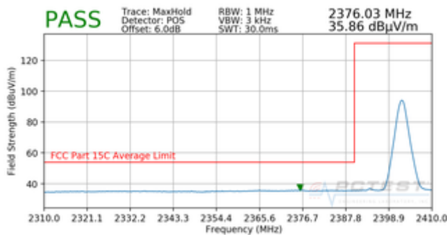
Plot 7-14. Radiated Restricted Lower Band Edge Measurement (Average)
