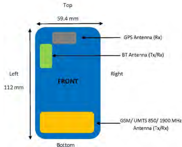
Figure 1-1 DUT Antenna Locations
