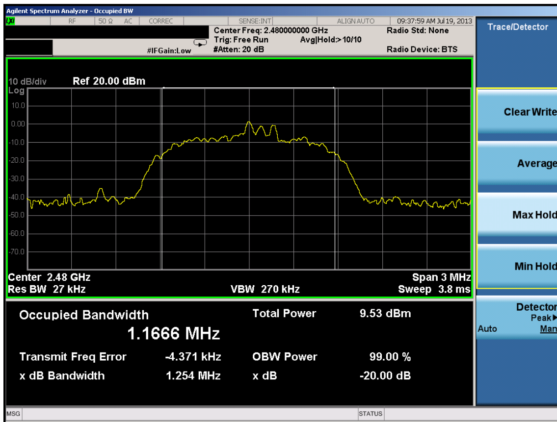
Plot 6-9. 20dB Bandwidth Plot (Bluetooth, 3Mbps – Ch. 78)
