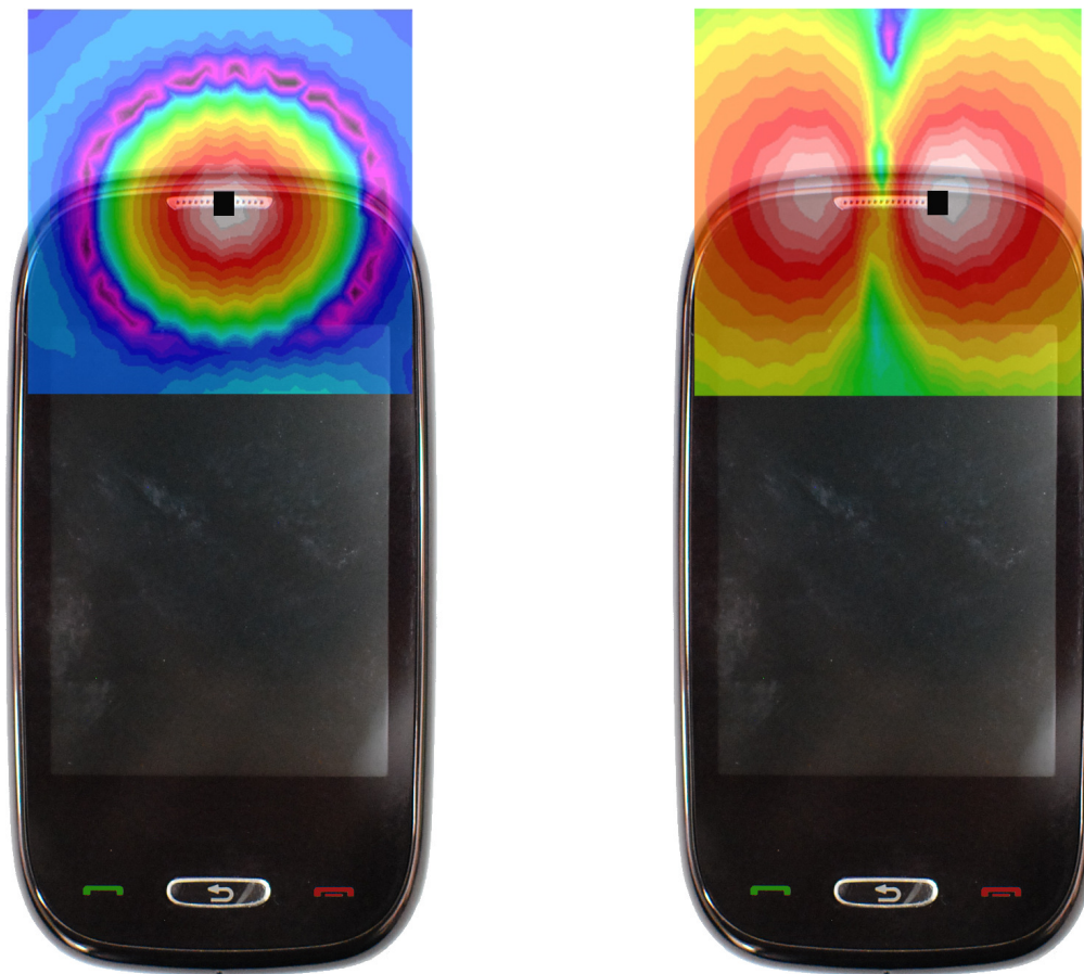
Figure 13-3 T-Coil Scan Overlay Magnetic Field Distributions
