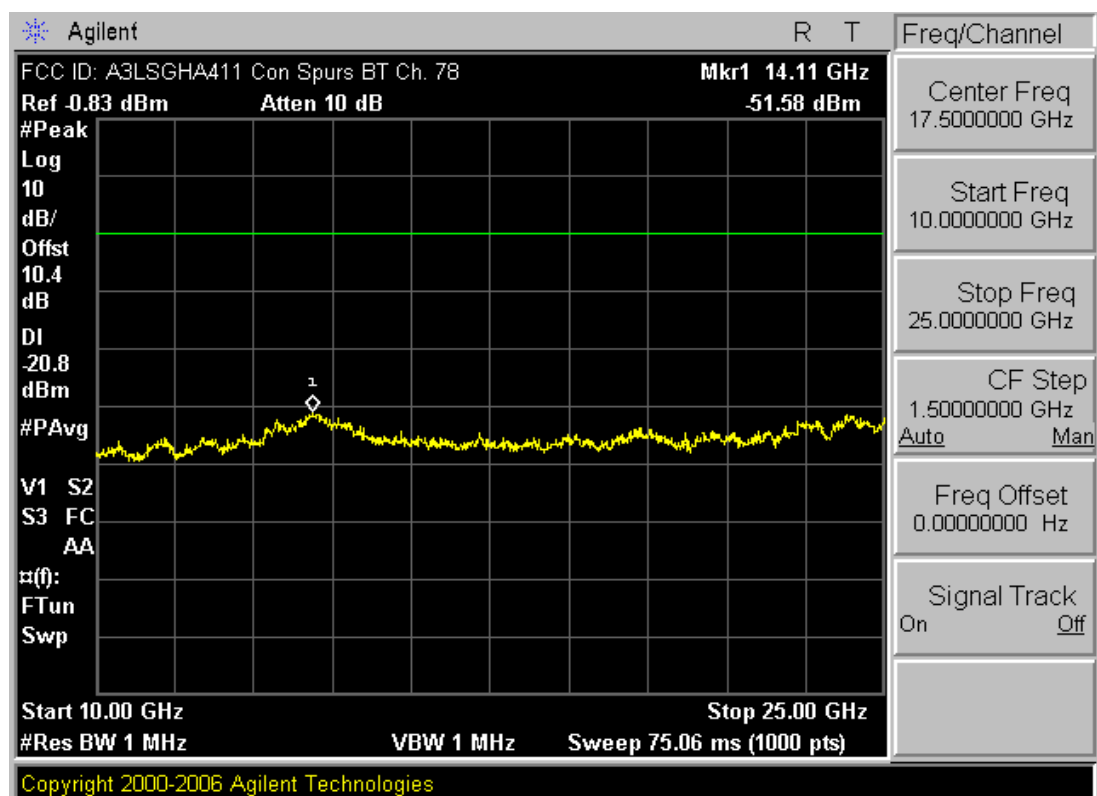
Plot 6-17. Conducted Spurious Plot (Bluetooth – Ch. 78)
