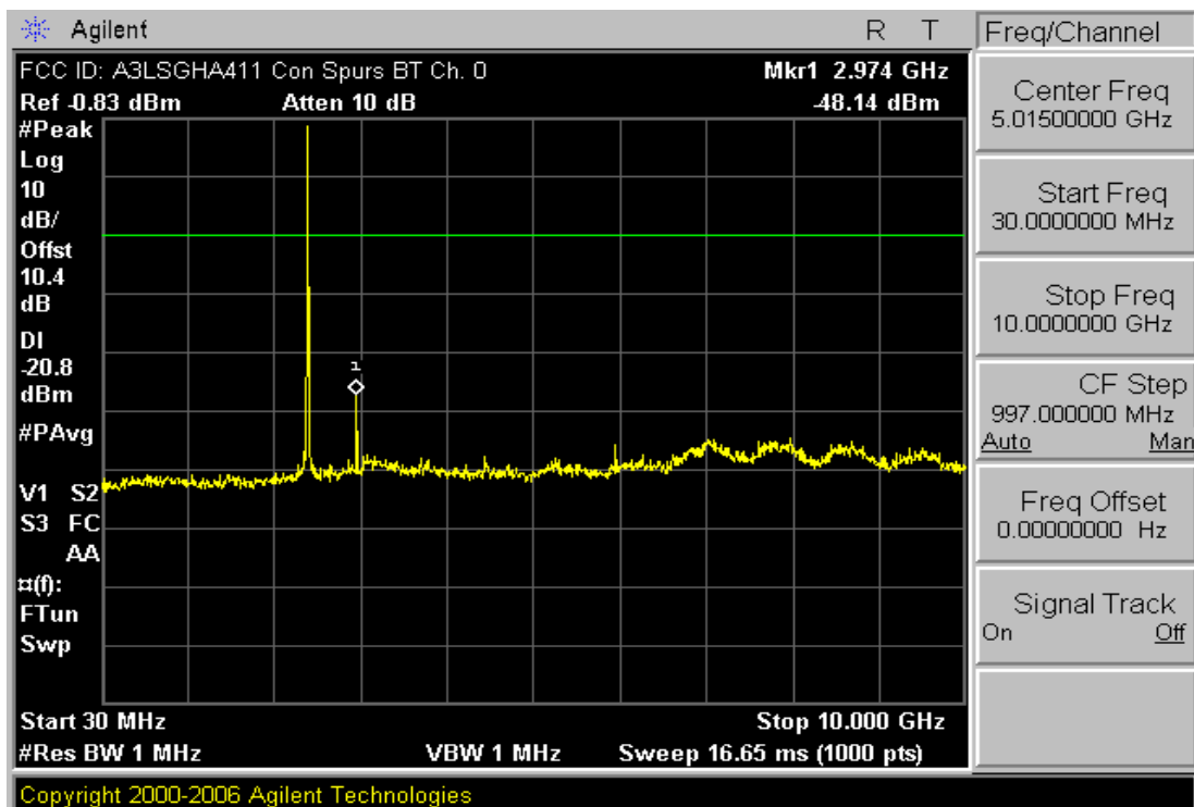
Plot 6-12. Conducted Spurious Plot (Bluetooth – Ch. 0)
