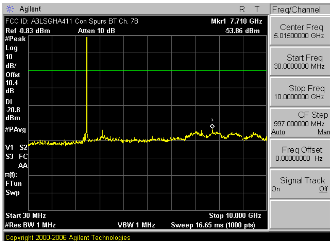
Plot 6-16. Conducted Spurious Plot (Bluetooth – Ch. 78)
