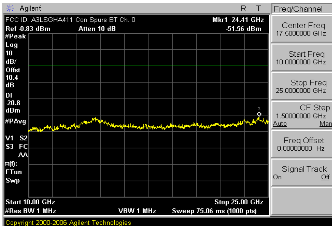
Plot 6-13. Conducted Spurious Plot (Bluetooth – Ch. 0)
