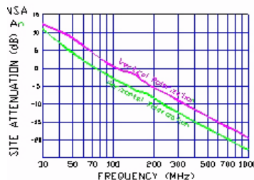
Figure 3.2-4. Normalized Site Attenuation Curves (H&V)
