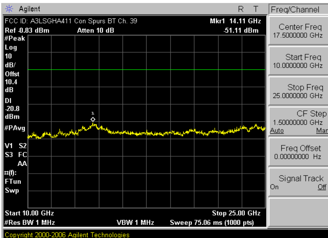
Plot 6-15. Conducted Spurious Plot (Bluetooth – Ch. 39)
