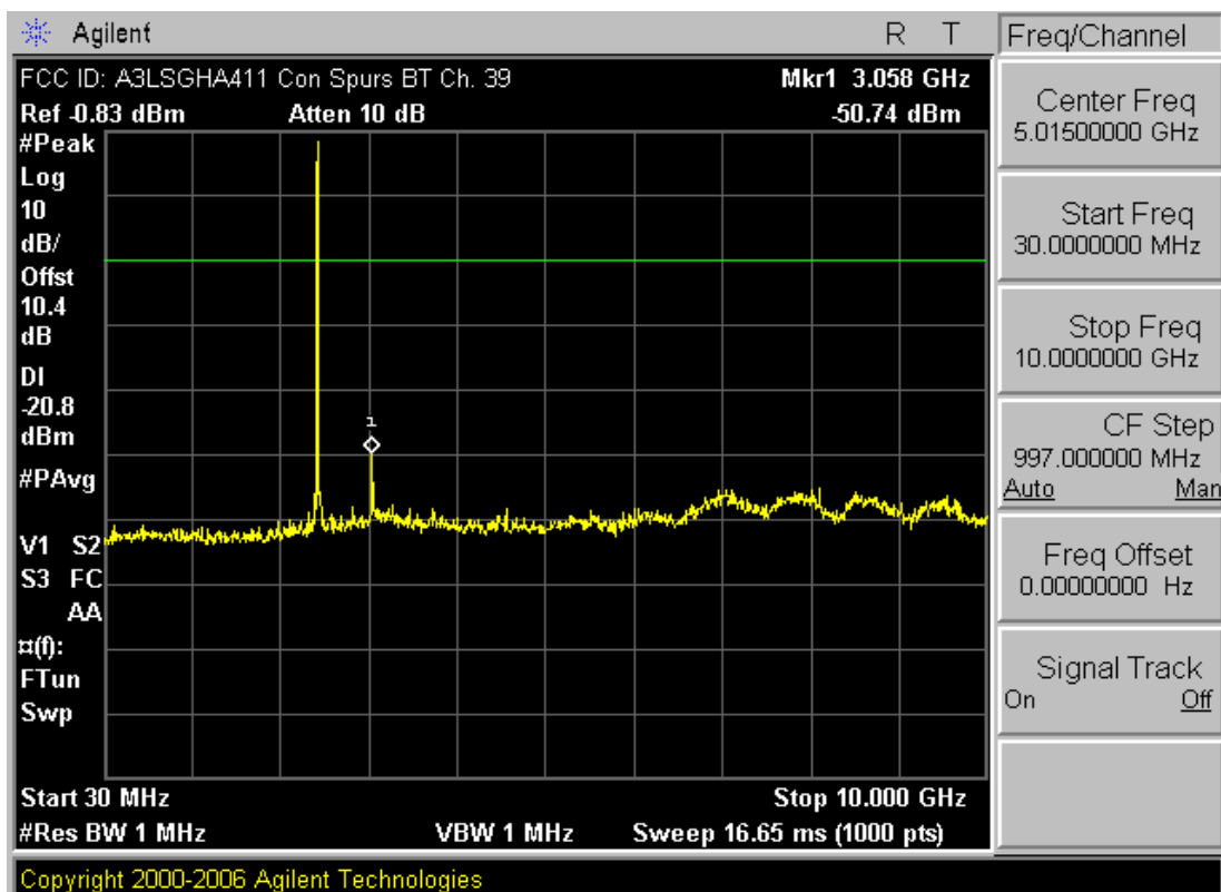
Plot 6-14. Conducted Spurious Plot (Bluetooth – Ch. 39)
