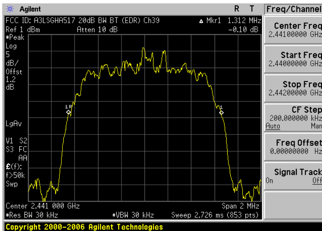
Plot 6-2. 20dB Bandwidth Plot (Bluetooth 2.0 with Enhanced Data Rate – Ch. 39)
