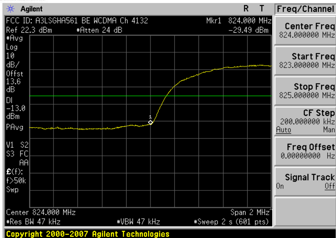
Plot 7-12. Band Edge Plot (Cellular WCDMA Mode – Ch. 4132)
