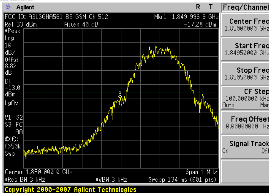
Plot 7-2. Band Edge Plot (PCS GSM Mode - Ch. 512)
