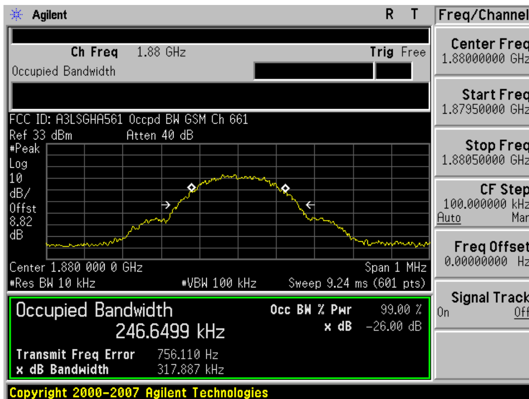
Plot 7-5. Occupied Bandwidth Plot (PCS GSM Mode – Ch. 661)
