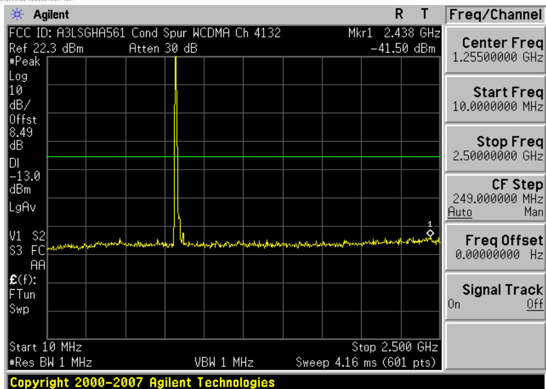
Plot 7-10. Conducted Spurious Plot (Cellular WCDMA Mode – Ch. 4132)
