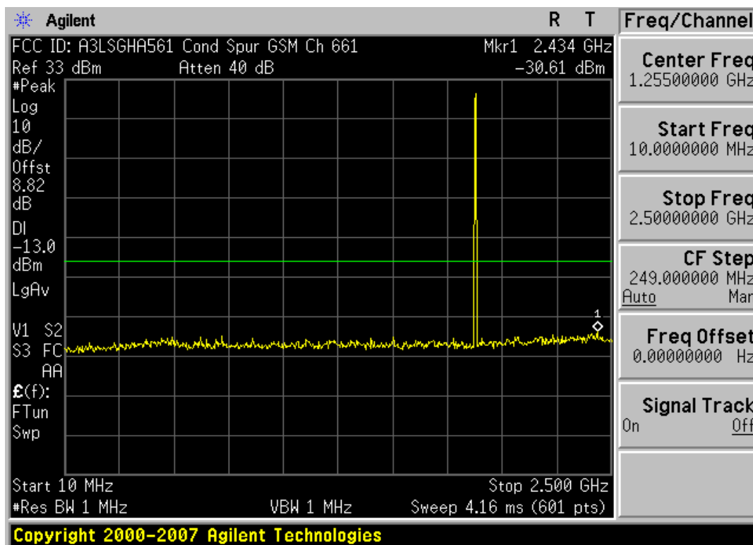
Plot 7-3. Conducted Spurious Plot (PCS GSM Mode - Ch. 661)
