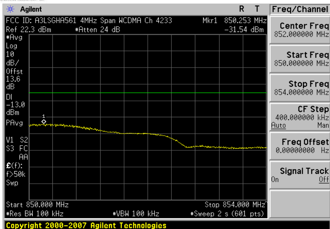
Plot 7-20. 4MHz Span Plot (Cellular WCDMA Mode – Ch. 4233)
