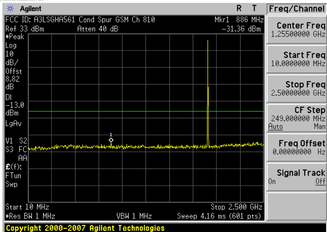
Plot 7-6. Conducted Spurious Plot (PCS GSM Mode – Ch. 810)
