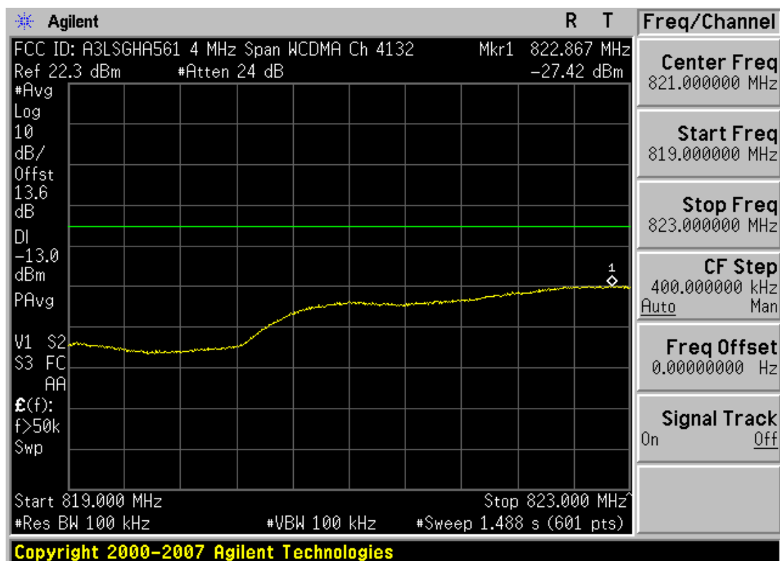
Plot 7-13. 4MHz Span Plot (Cellular WCDMA Mode – Ch. 4132)
