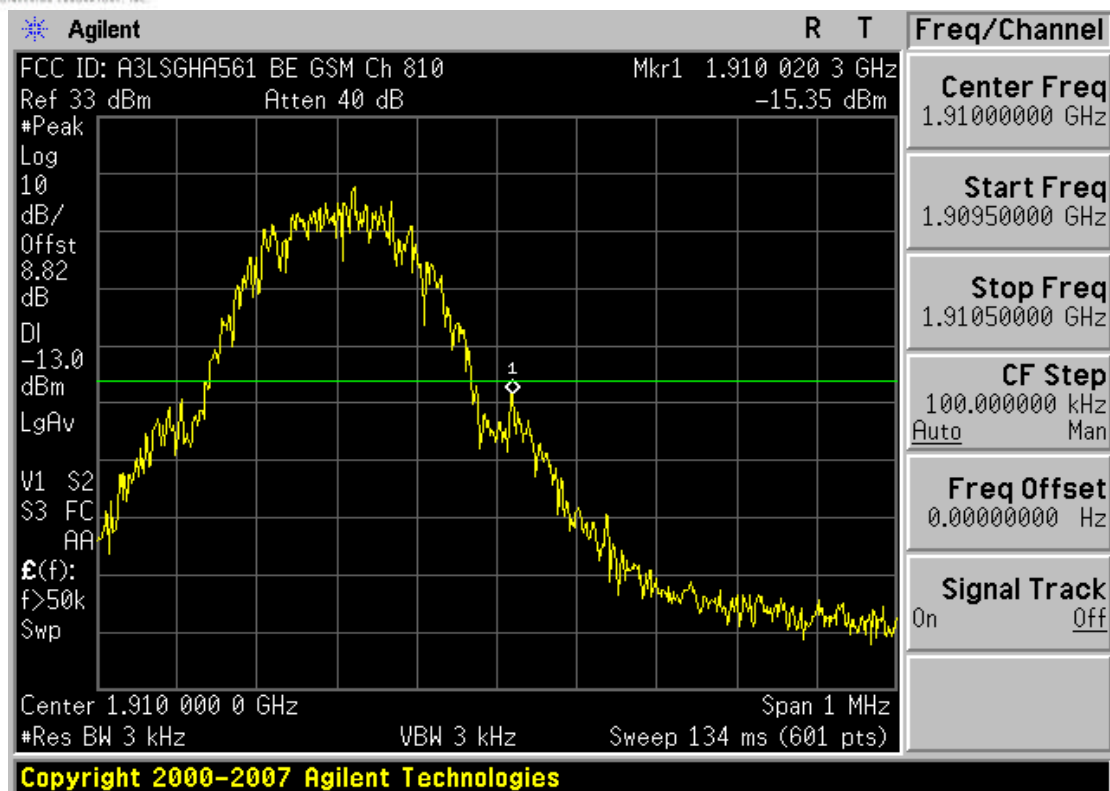
Plot 7-8. Band Edge Plot (PCS GSM Mode – Ch. 810)
