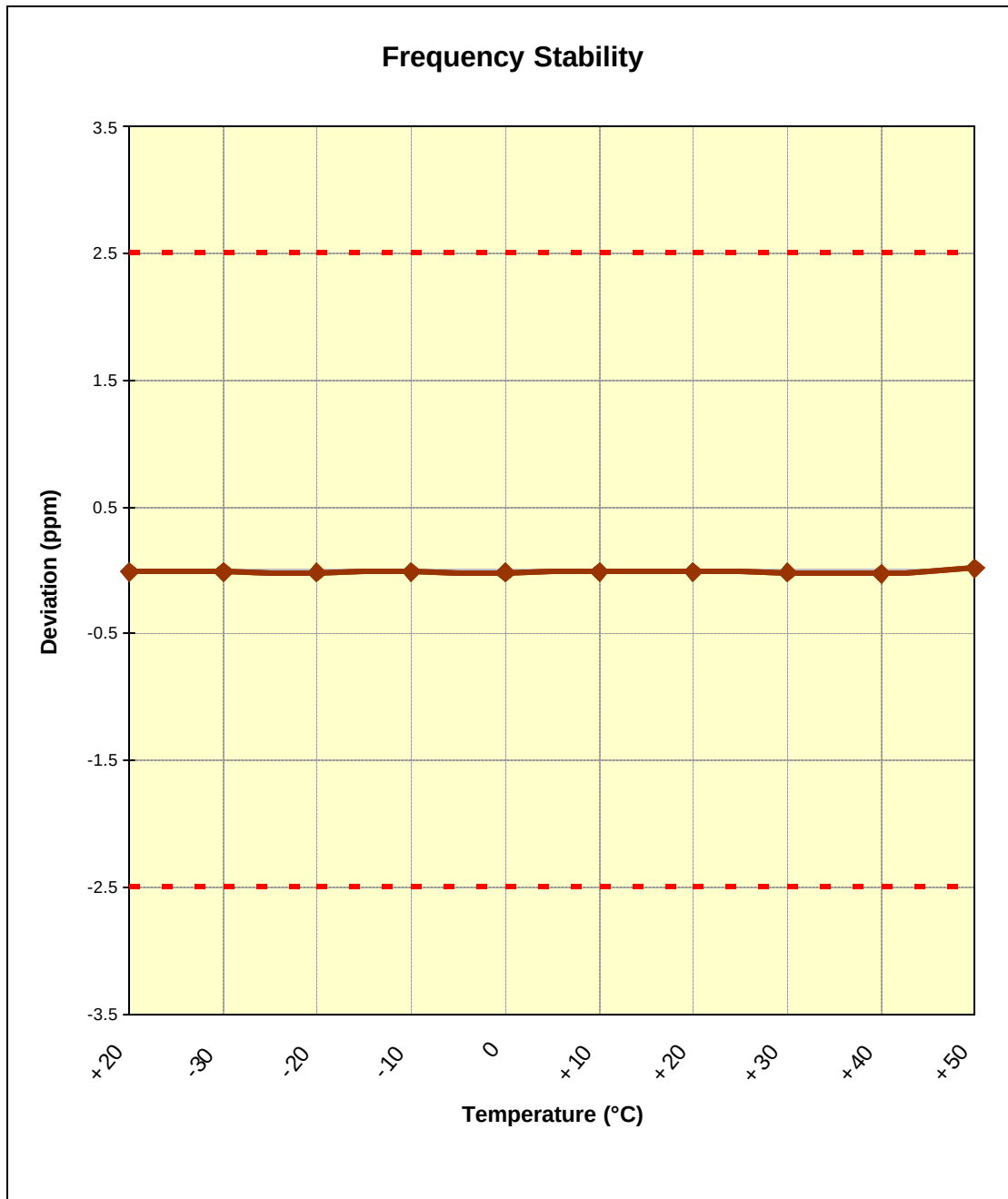
Plot 6-1. Frequency Stability Graph (Cellular WCDMA Mode – Ch. 4183)
