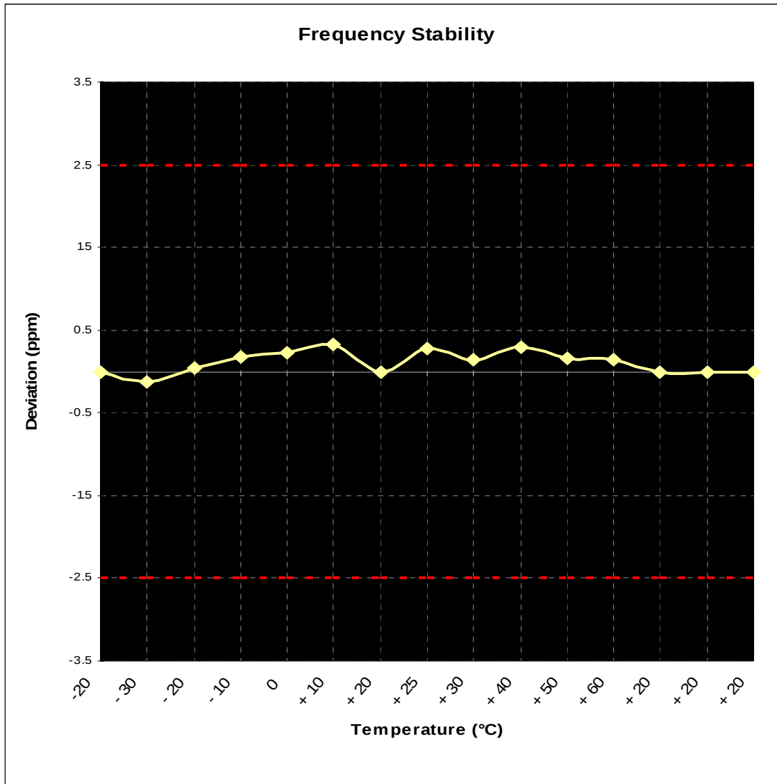
Plot 6-1. Frequency Stability Graph (Cellular GSM Mode – Ch. 190)
