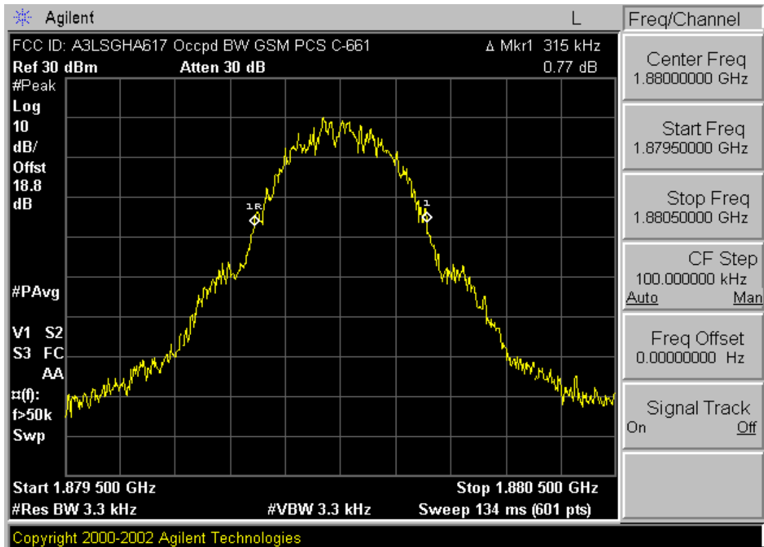
Plot A-16. Occupied Bandwidth Plot (PCS GSM Mode – Ch. 661)
