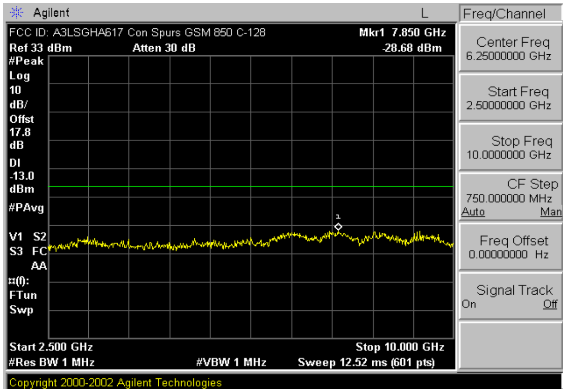
Plot A-2. Conducted Spurious Plot (Cellular GSM Mode – Ch. 128)
