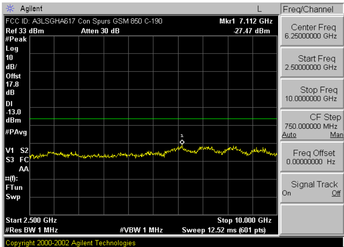
Plot A-5. Conducted Spurious Plot (Cellular GSM Mode – Ch. 190)
