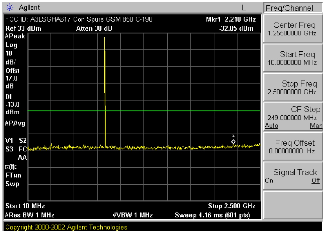
Plot A-4. Conducted Spurious (Cellular GSM Mode – Ch. 190)
