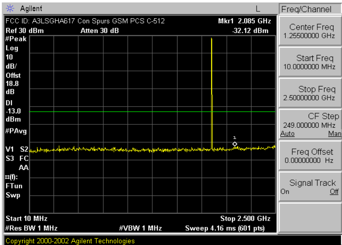
Plot A-11. Conducted Spurious Plot (PCS GSM Mode – Ch. 512)
