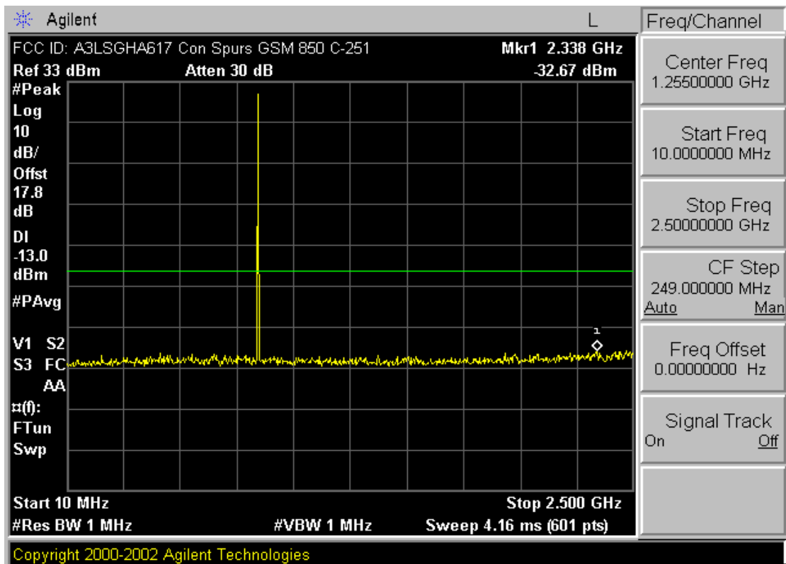
Plot A-7. Conducted Spurious Plot (Cellular GSM Mode – Ch. 251)
