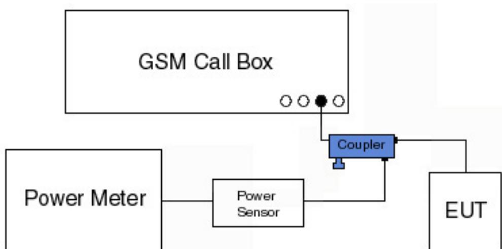
Figure 6-1. GSM Conducted Power Test Setup Diagram
