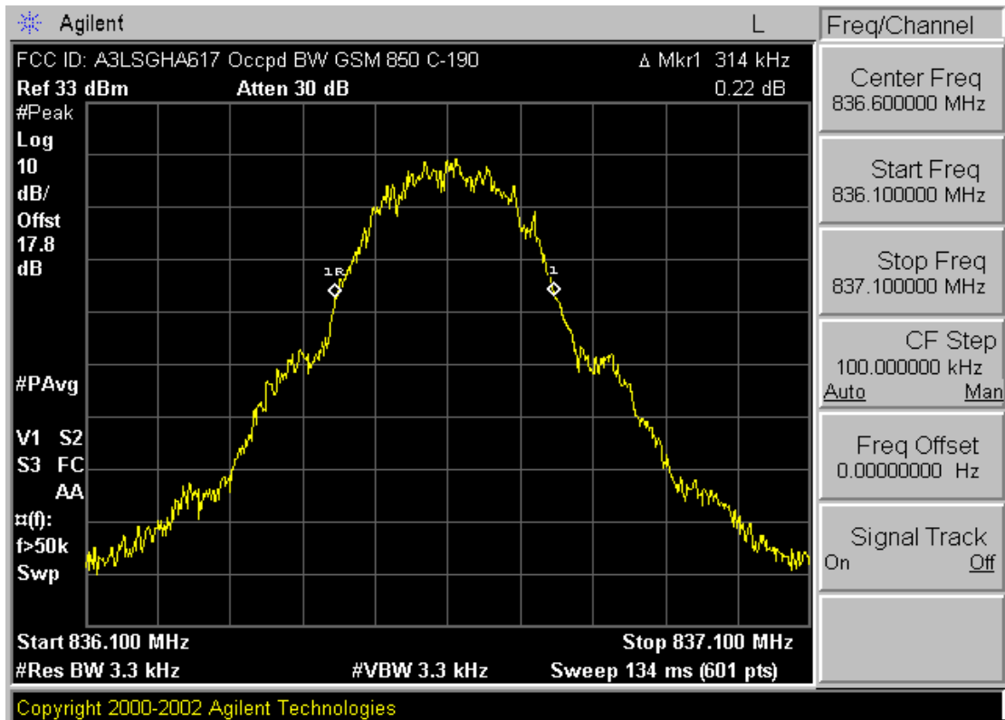
Plot A-6. Occupied Bandwidth Plot (Cellular GSM Mode – Ch. 190)
