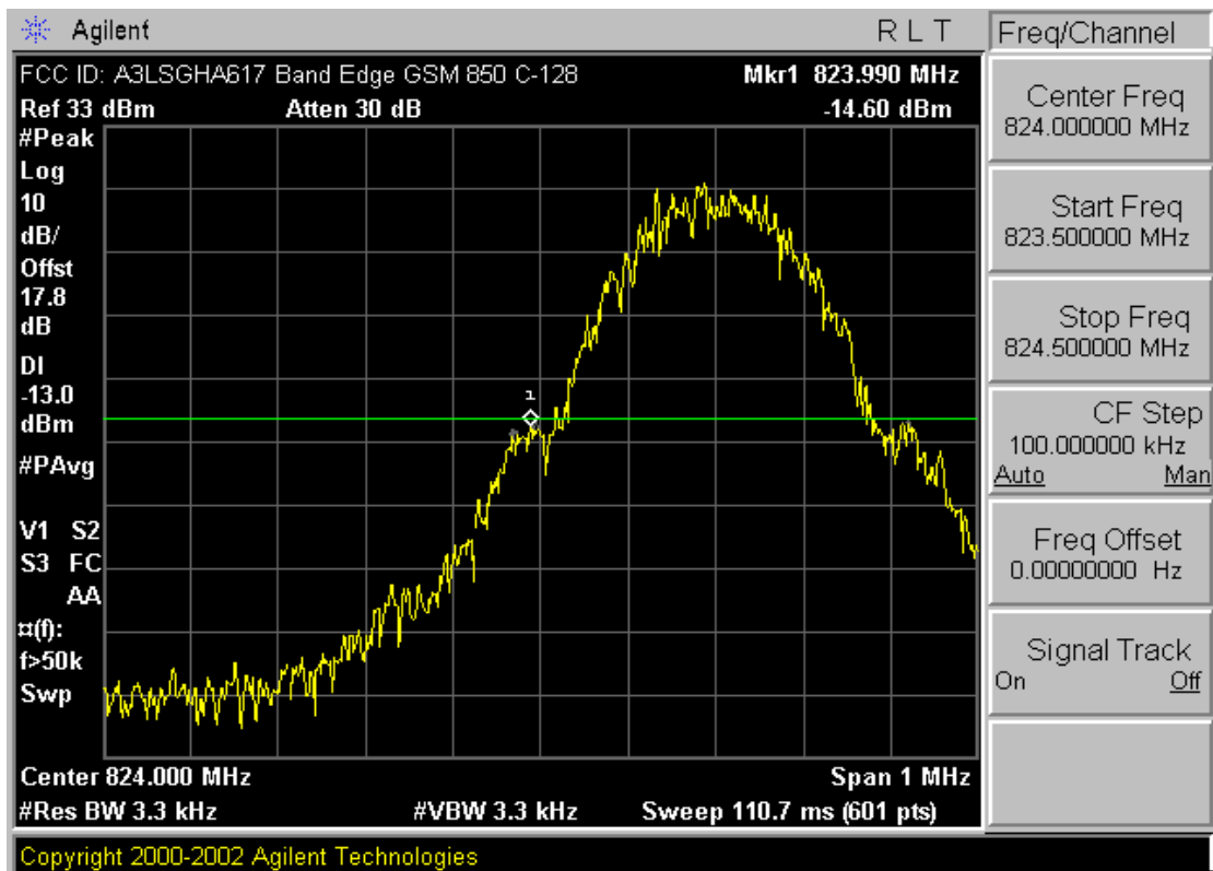
Plot A-3. Band Edge Plot (Cellular GSM Mode – Ch. 128)
