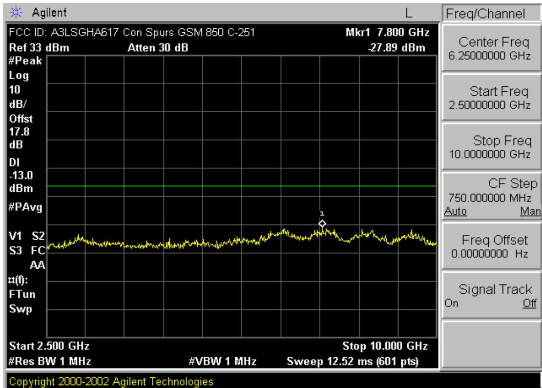
Plot A-8. Conducted Spurious Plot (Cellular GSM Mode – Ch. 251)
