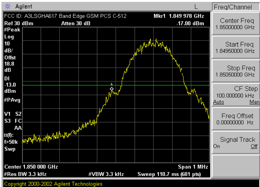
Plot A-13. Band Edge Plot (PCS GSM Mode – Ch. 512)
