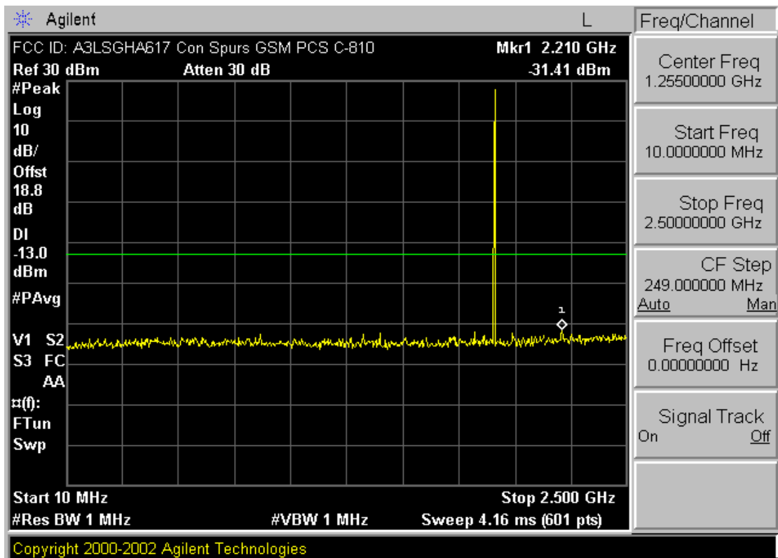
Plot A-17. Conducted Spurious Plot (PCS GSM Mode – Ch. 810)
