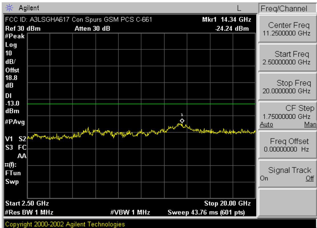
Plot A-15. Conducted Spurious Plot (PCS GSM Mode – Ch. 661)
