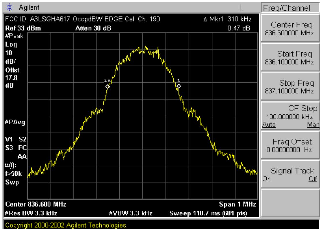
Plot A-10. Occupied Bandwidth Plot (EDGE850 Mode – Ch. 190)
