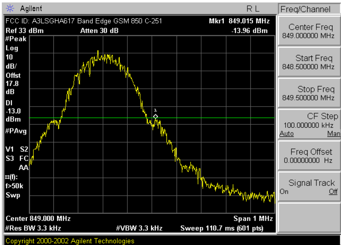
Plot A-9. Band Edge Plot (Cellular GSM Mode – Ch. 251)
