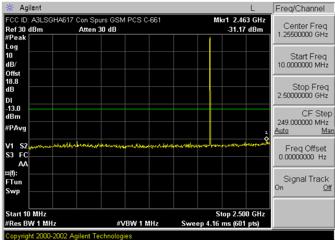
Plot A-14. Conducted Spurious Plot (PCS GSM Mode – Ch. 661)
