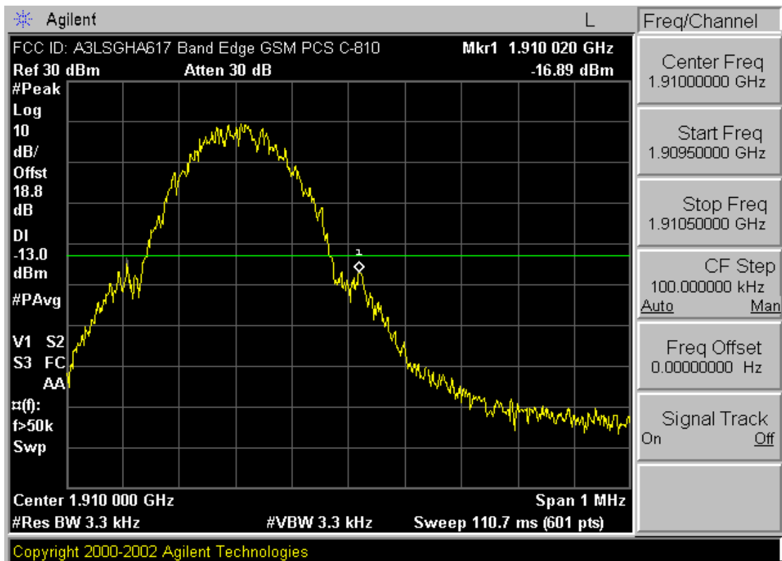
Plot A-19. Band Edge Plot (PCS GSM Mode – Ch. 810)
