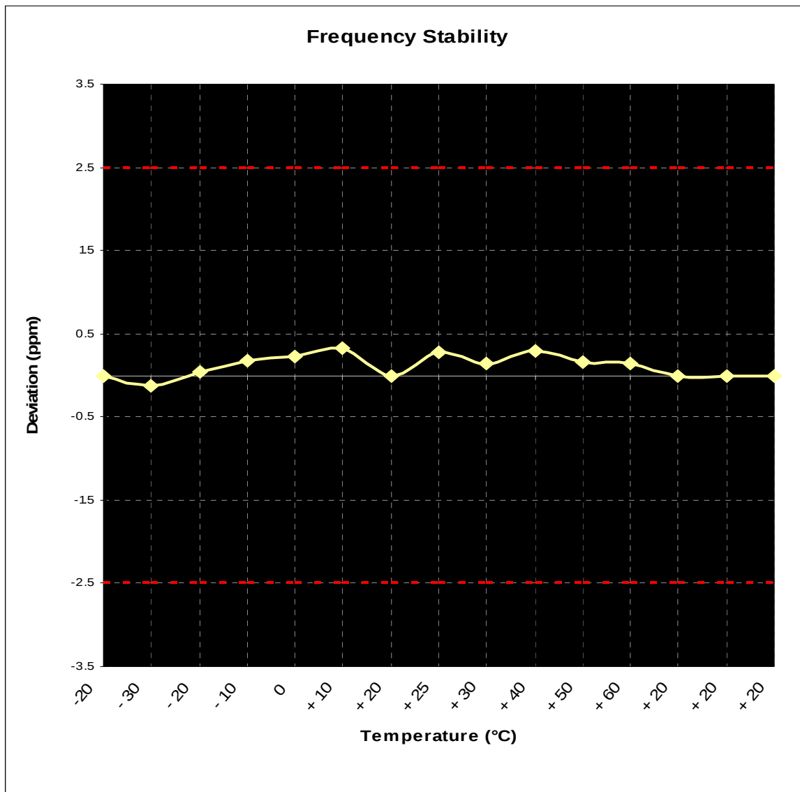
Plot 6-2. Frequency Stability Graph (PCS GSM Mode – Ch. 661)
