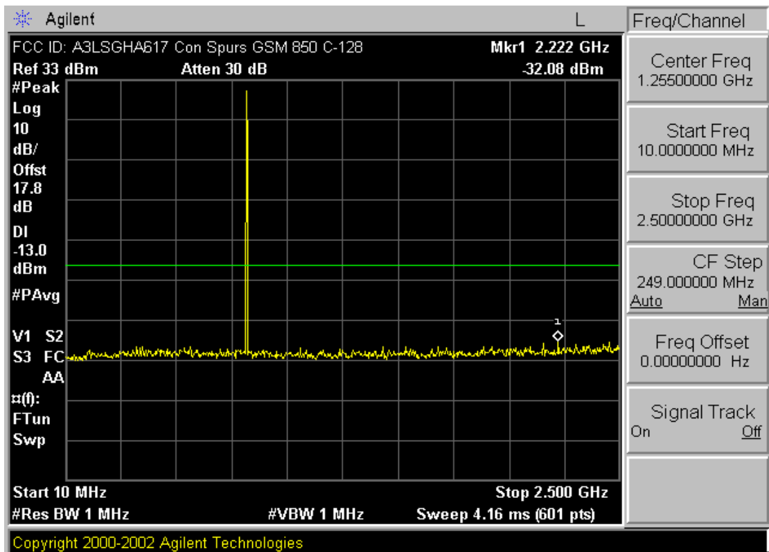
Plot A-1. Conducted Spurious Plot (Cellular GSM Mode – Ch. 128)
