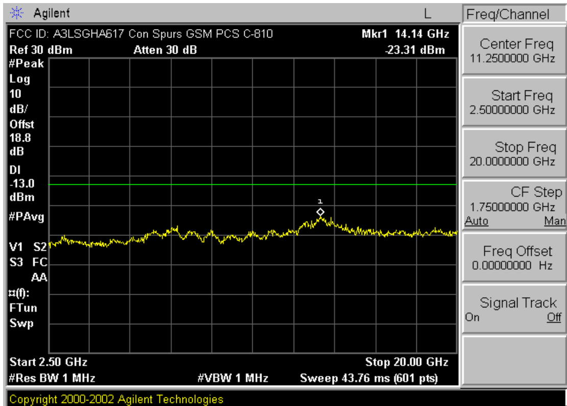
Plot A-18. Conducted Spurious Plot (PCS GSM Mode – Ch. 810)
