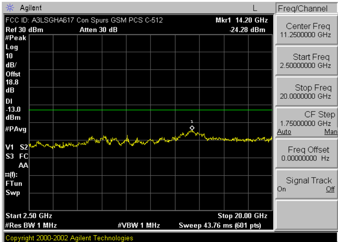
Plot A-12. Conducted Spurious Plot (PCS GSM Mode – Ch. 512)
