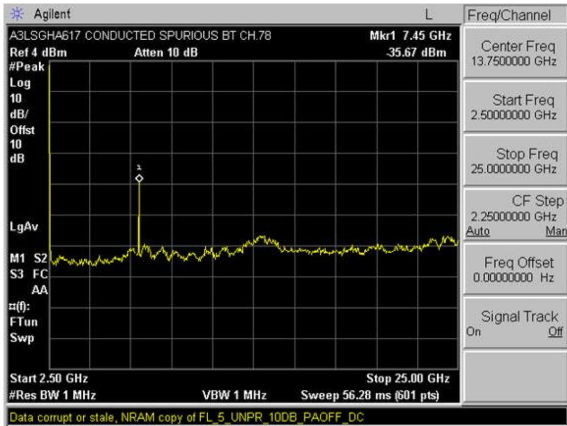
Plot 6-15. Conducted Spurious Plot (Bluetooth – Ch. 78)
