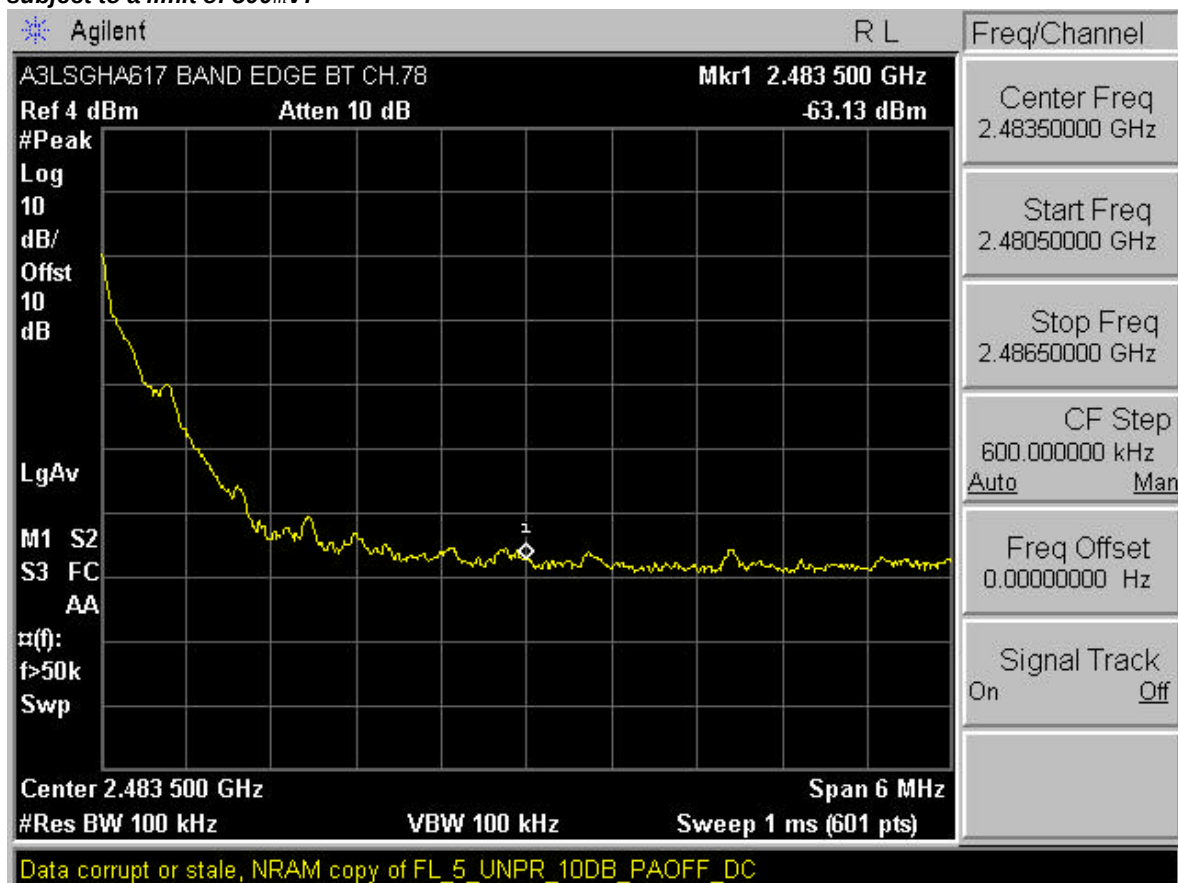
Plot 6-4. Band Edge Plot (Bluetooth – Ch. 78)
