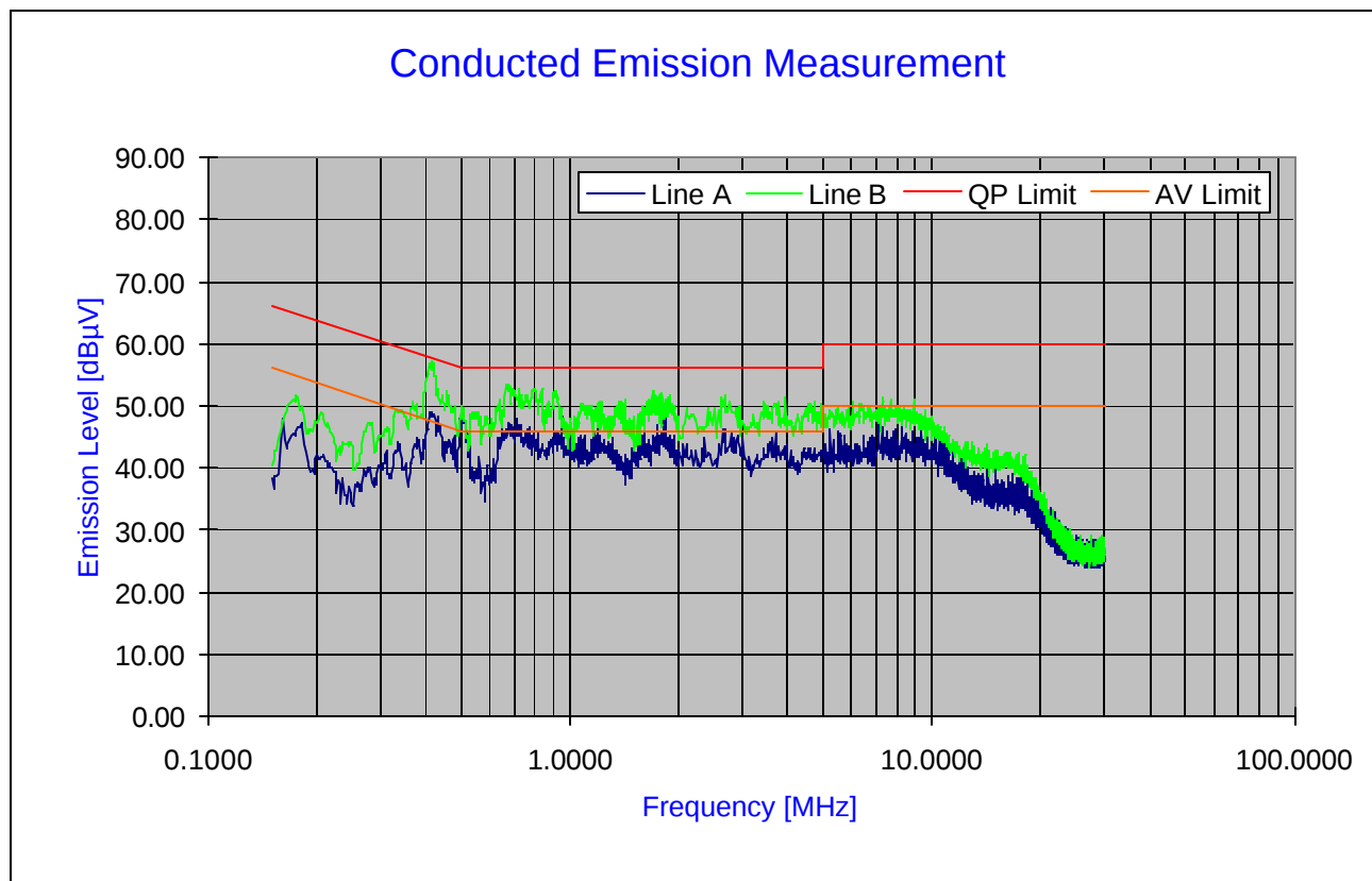
Plot 6-16. Line Conducted Plot with Bluetooth
