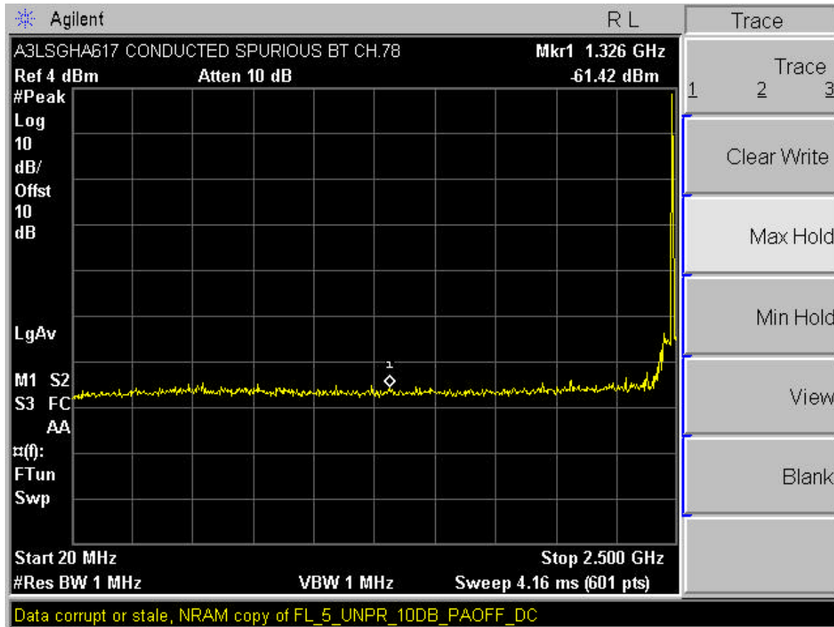
Plot 6-14. Conducted Spurious Plot (Bluetooth – Ch. 78)
