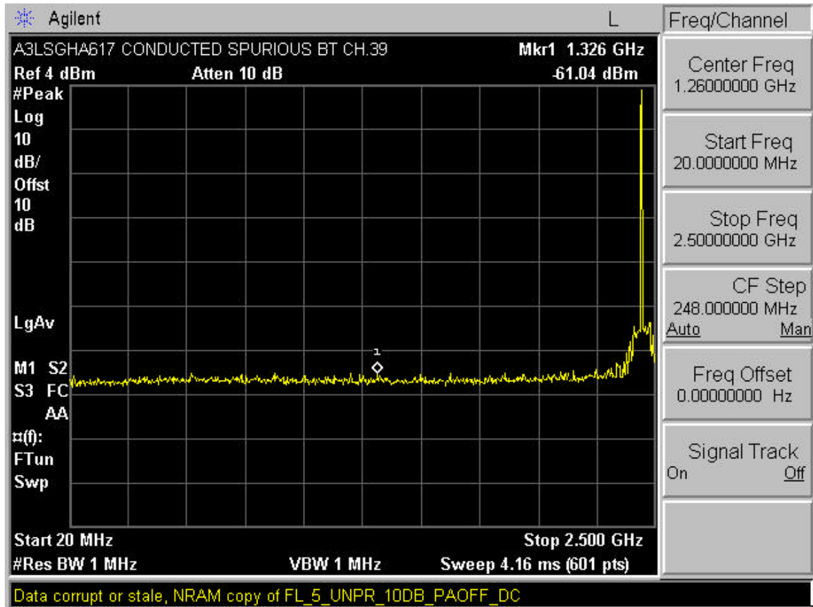
Plot 6-12. Conducted Spurious Plot (Bluetooth – Ch. 39)
