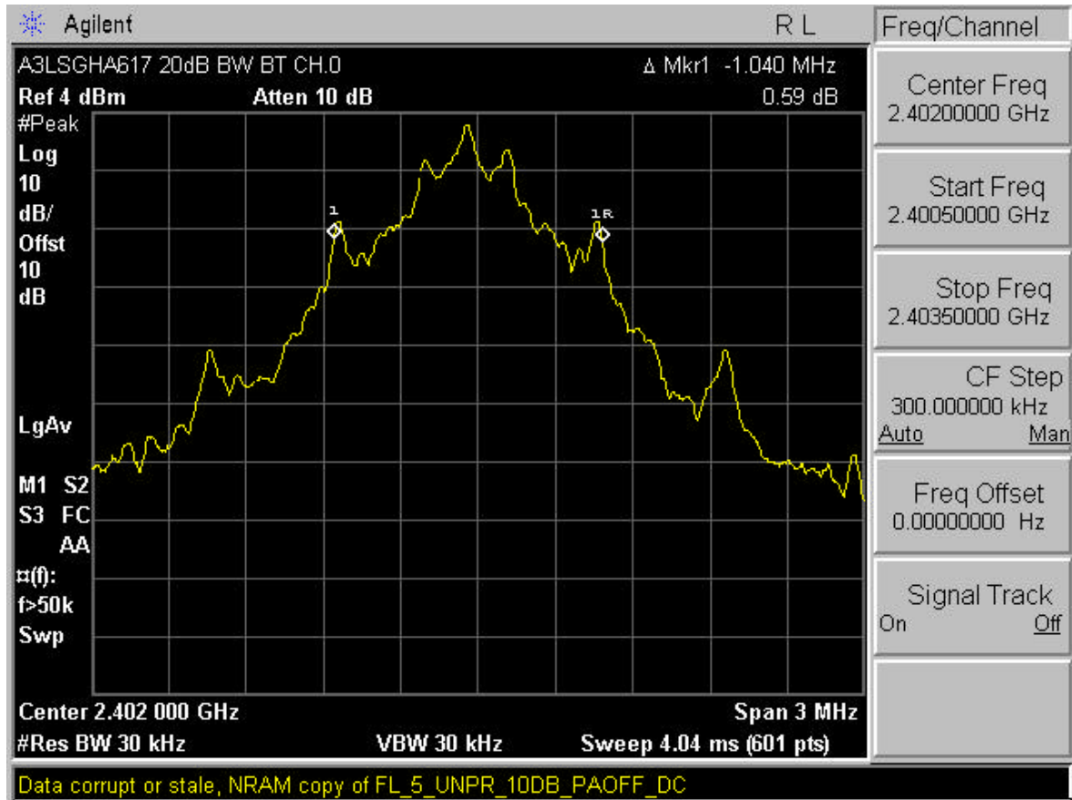
Plot 6-1. 20dB Bandwidth Plot (Bluetooth – Ch. 0)
