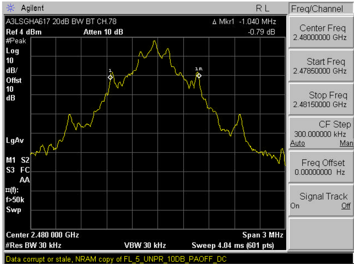
Plot 6-3. 20dB Bandwidth Plot (Bluetooth – Ch. 78)
