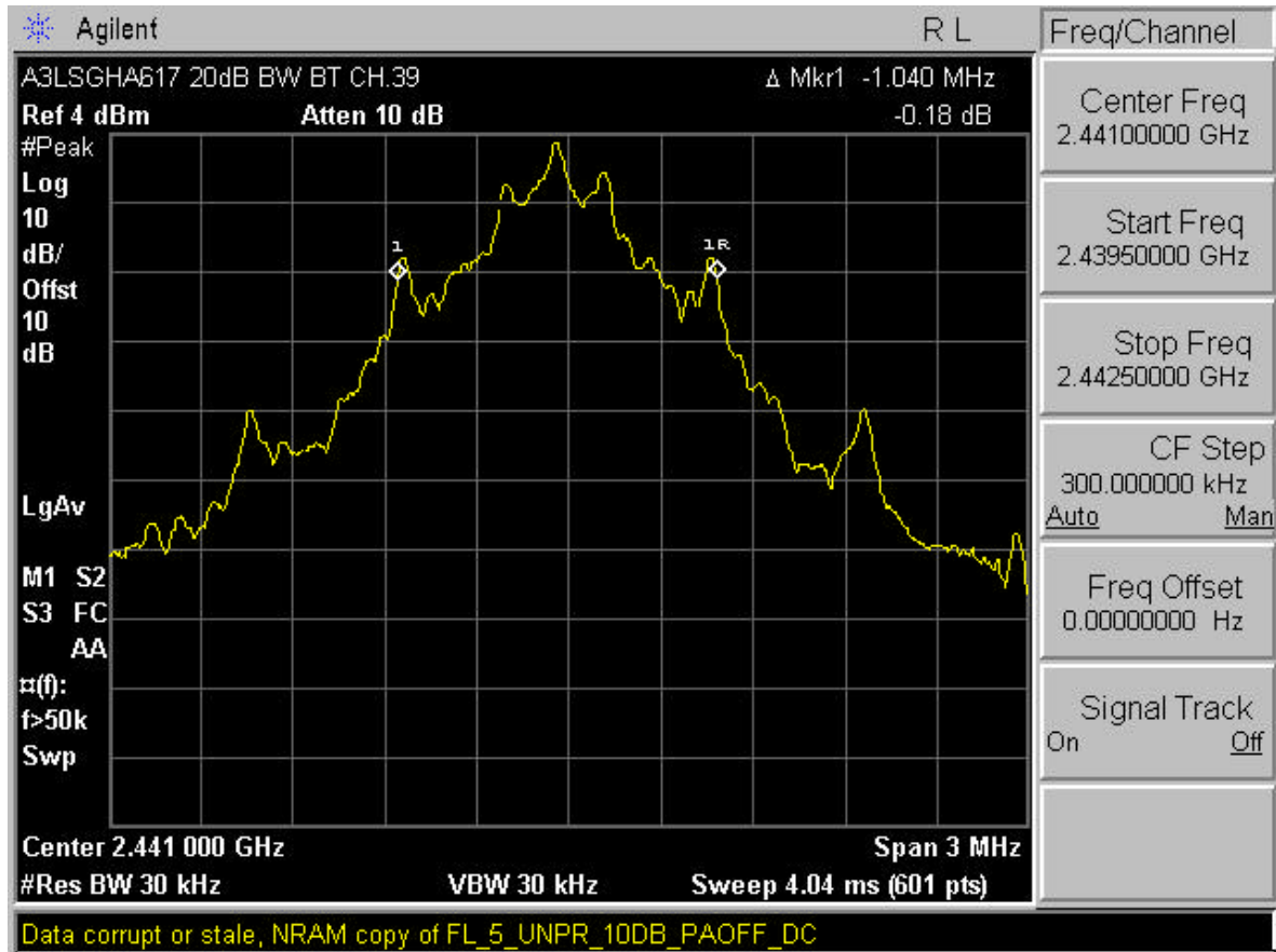
Plot 6-2. 20dB Bandwidth Plot (Bluetooth – Ch. 39)
