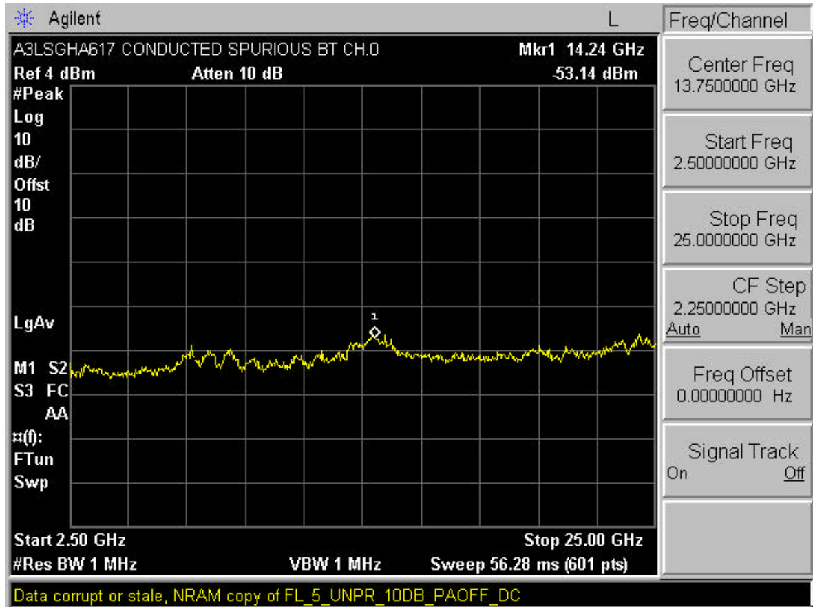
Plot 6-11. Conducted Spurious Plot (Bluetooth – Ch. 0)
