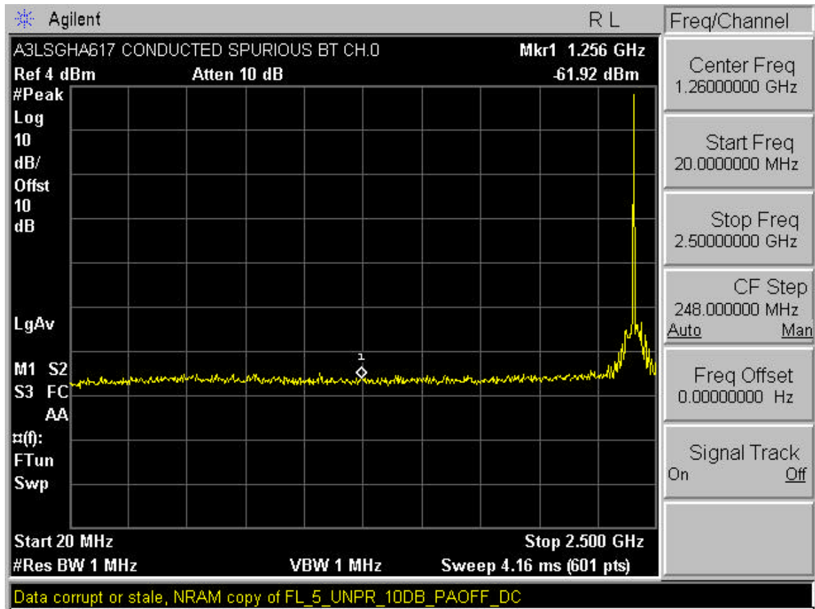
Plot 6-10. Conducted Spurious Plot (Bluetooth – Ch. 0)
