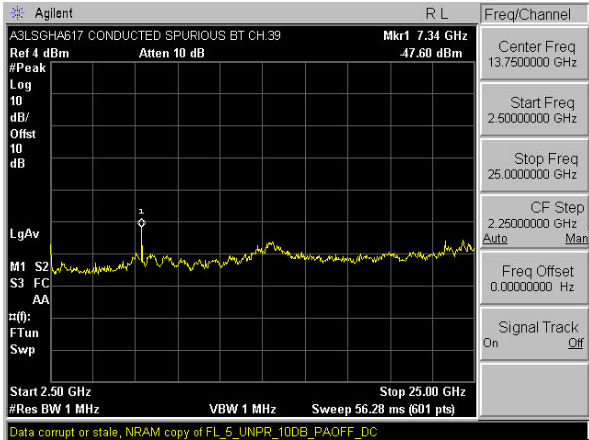
Plot 6-13. Conducted Spurious Plot (Bluetooth – Ch. 39)
