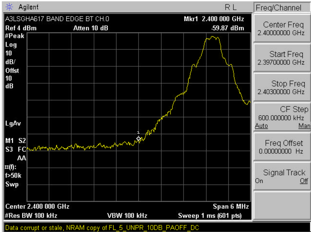
Plot 6-5. Band Edge Plot (Bluetooth – Ch. 0)
