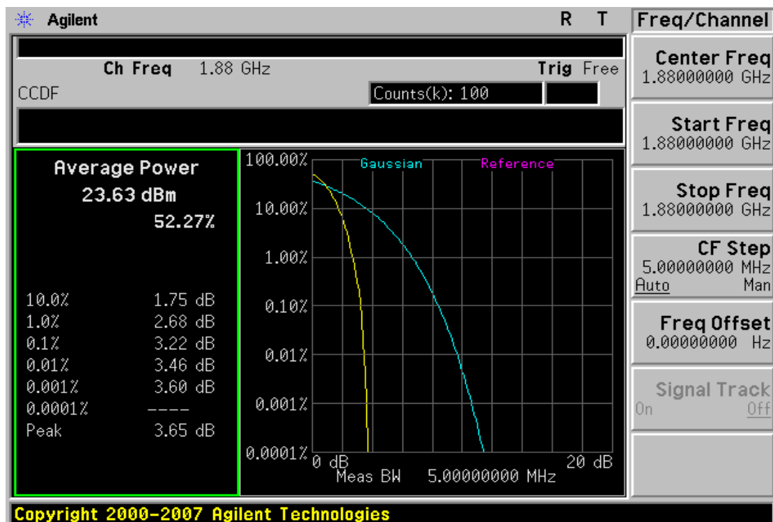
Plot 7-41. Peak-Average Ratio Plot (PCS WCDMA Mode – Ch. 9400)
