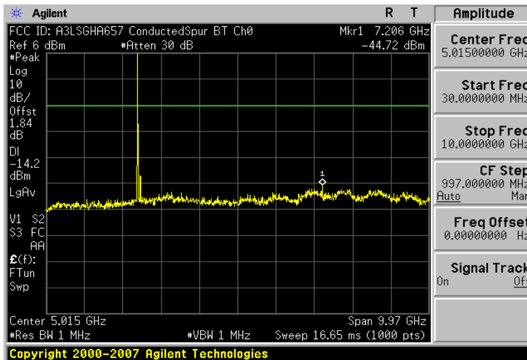
Plot 6-12. Conducted Spurious Plot (Bluetooth – Ch. 0)
