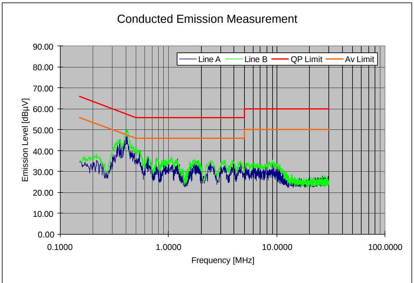
Plot 6-18. Line Conducted Plot with Bluetooth
