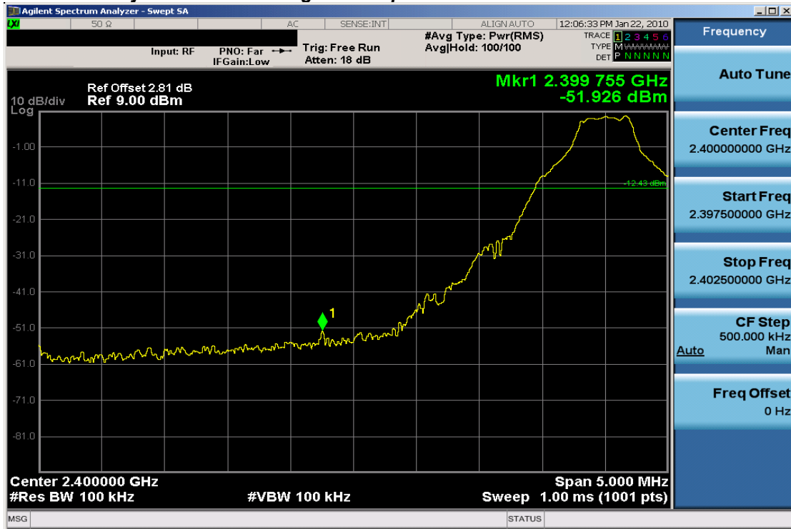
Plot 6-4. Band Edge Plot (Bluetooth – Ch. 0)
