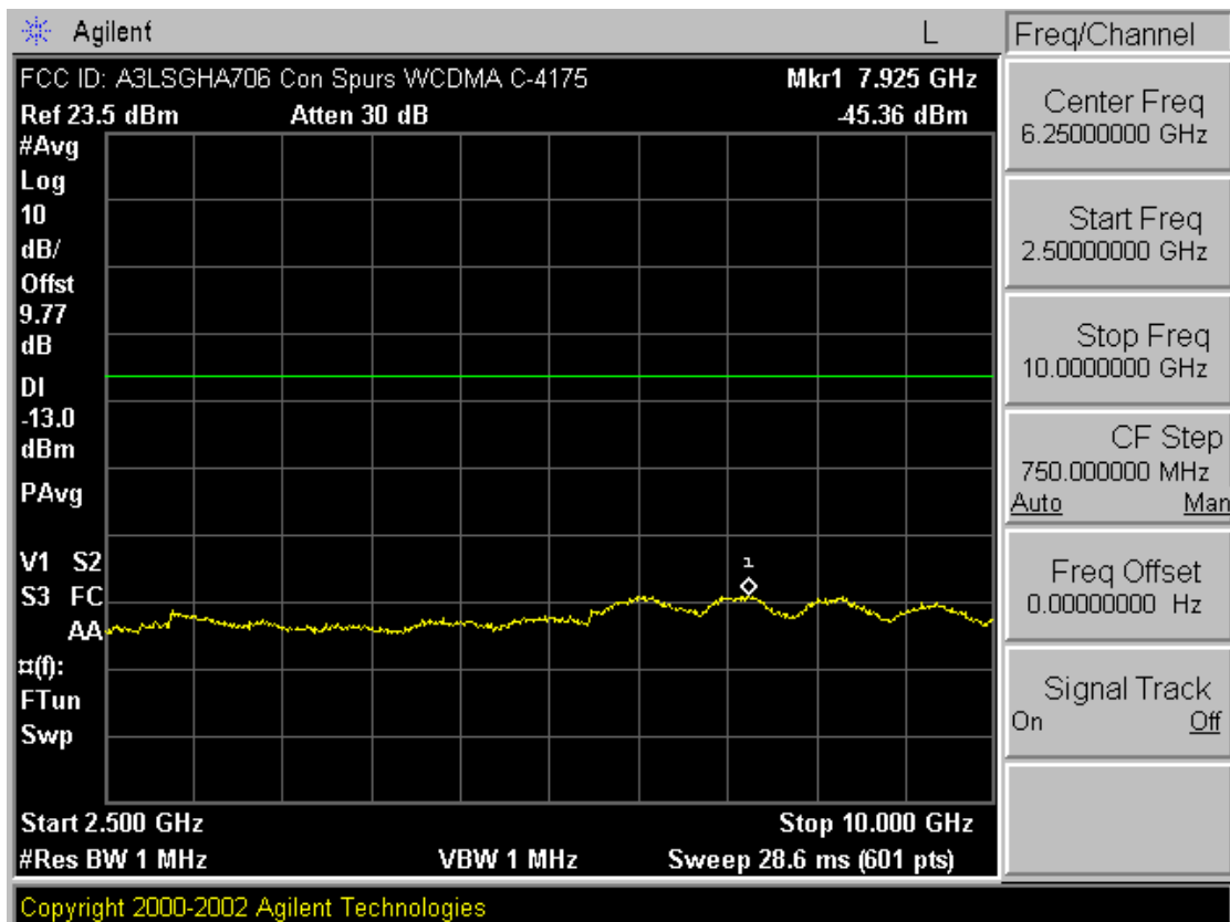
Plot A-6. Conducted Spurious Plot (Cellular WCDMA Mode – Ch. 4175)
