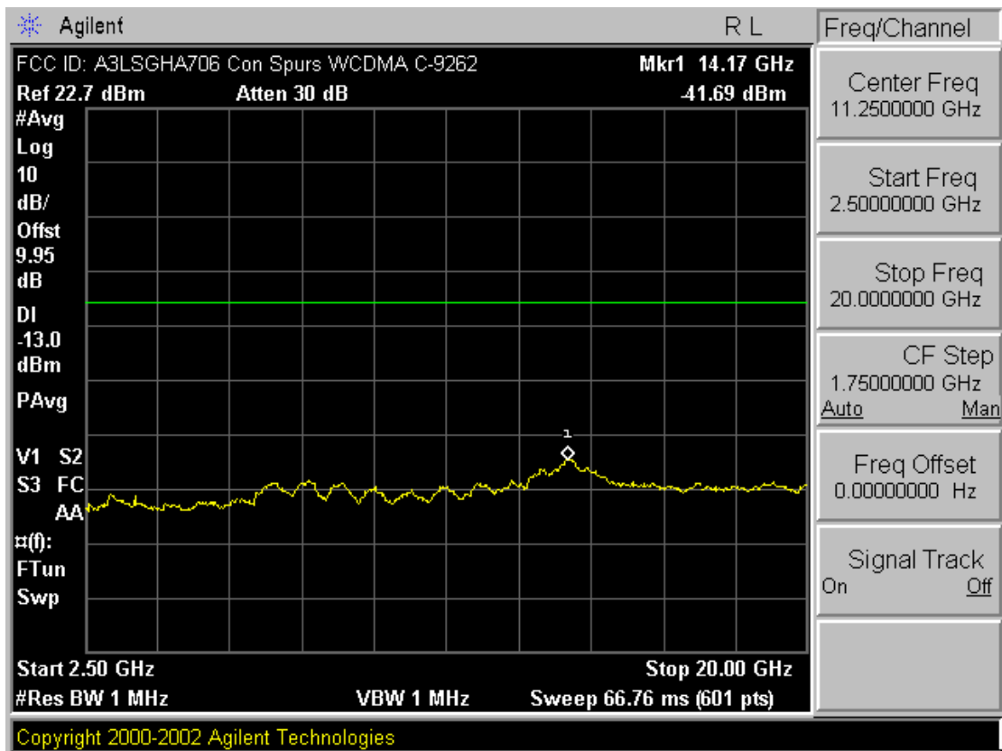
Plot A-13. Conducted Spurious Plot (PCS WCDMA Mode – Ch. 9262)
