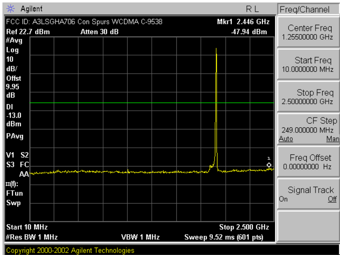
Plot A-19. Conducted Spurious Plot (PCS WCDMA Mode – Ch. 9538)
