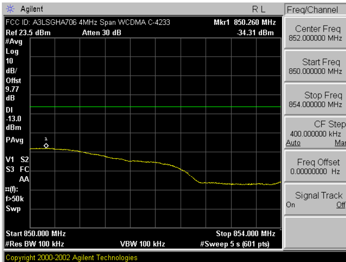
Plot A-11. 4MHz Span Plot (Cellular WCDMA Mode – Ch. 4233)
