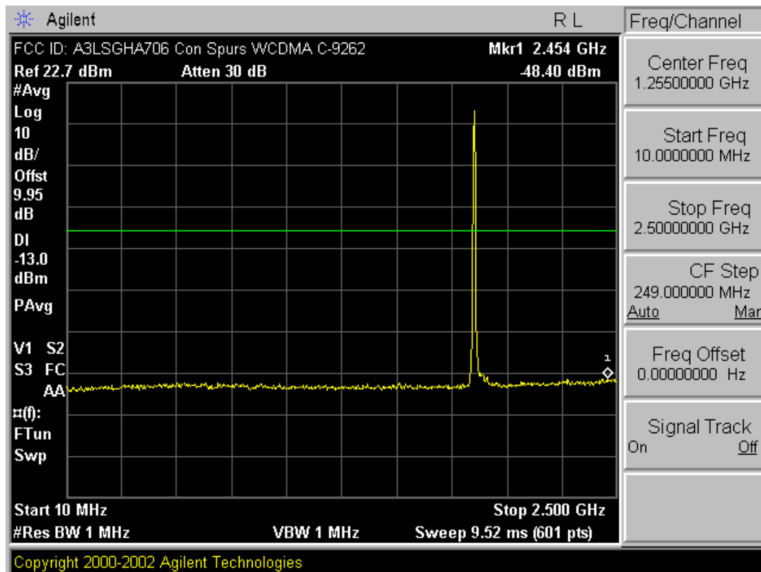
Plot A-12. Conducted Spurious Plot (PCS WCDMA Mode – Ch. 9262)
