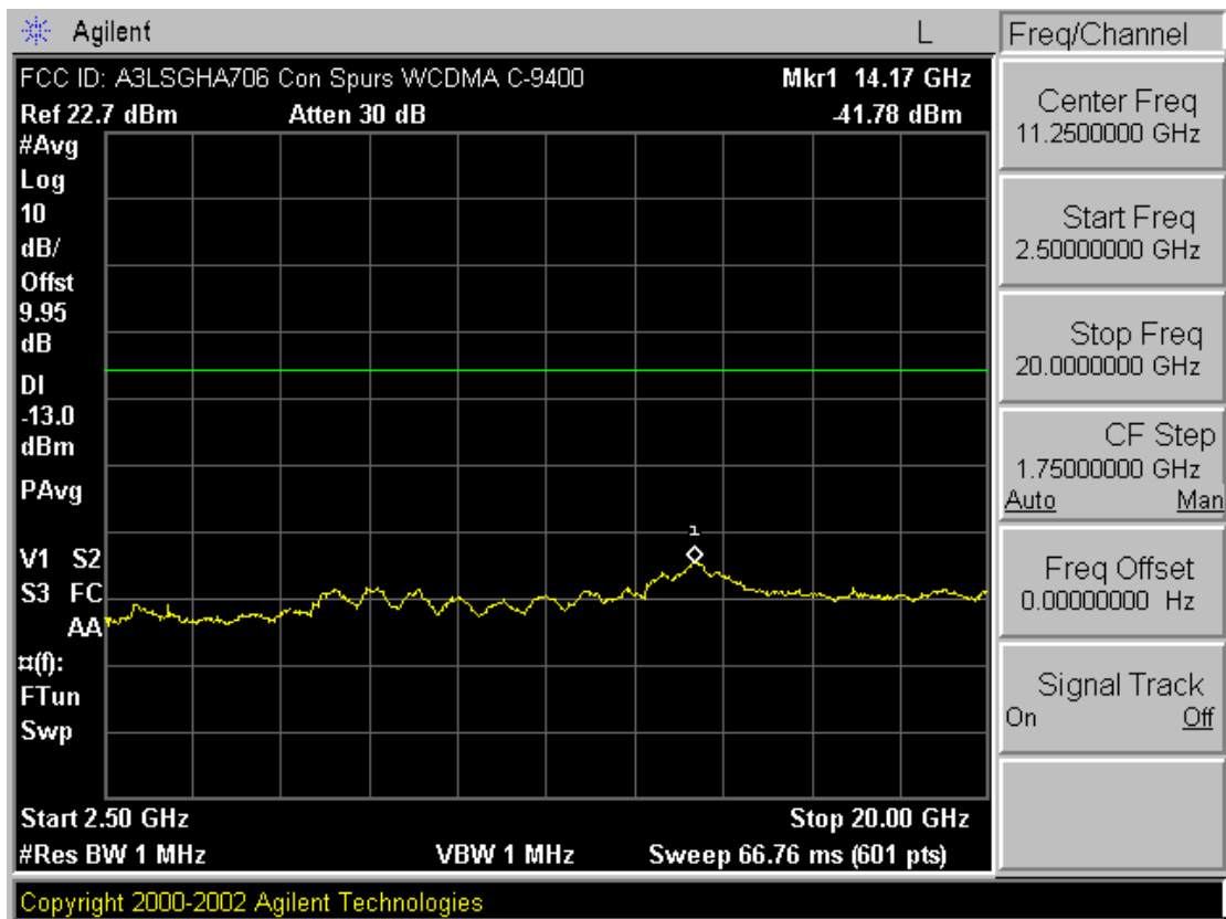
Plot A-17. Conducted Spurious Plot (PCS WCDMA Mode – Ch. 9400)
