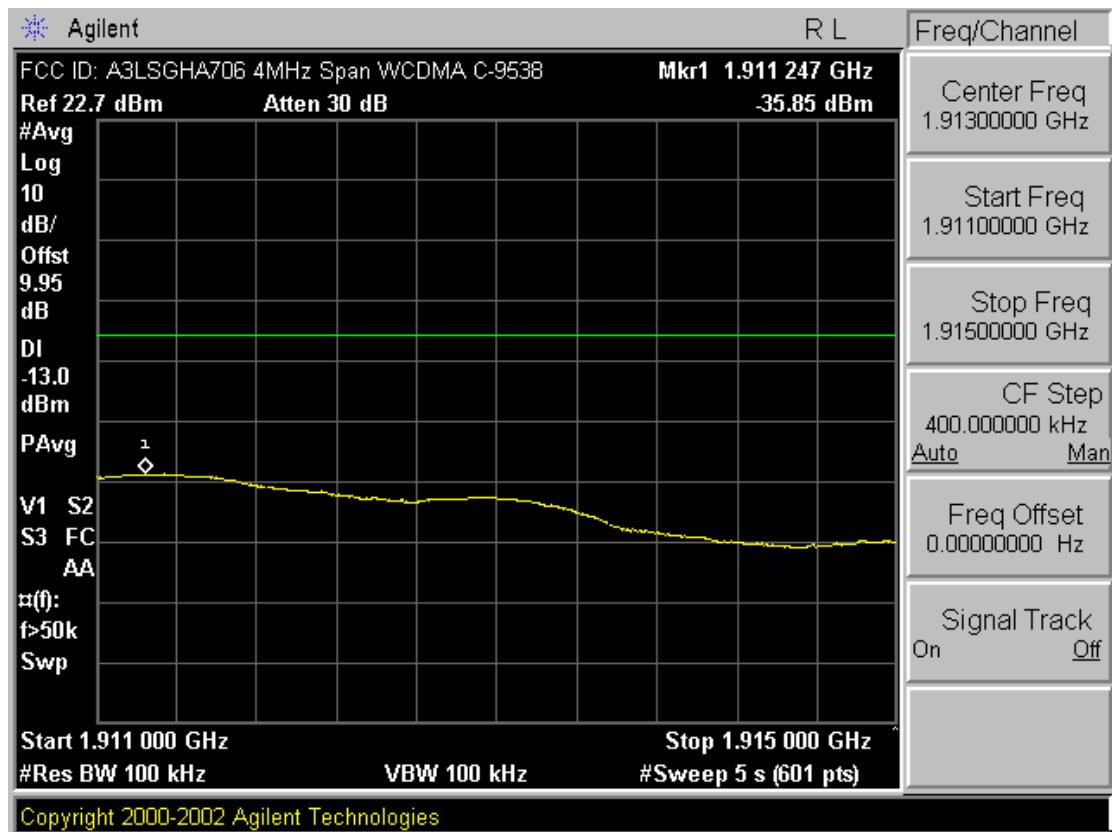
Plot A-22. 4MHz Span Plot (PCS WCDMA Mode – Ch. 9538)
