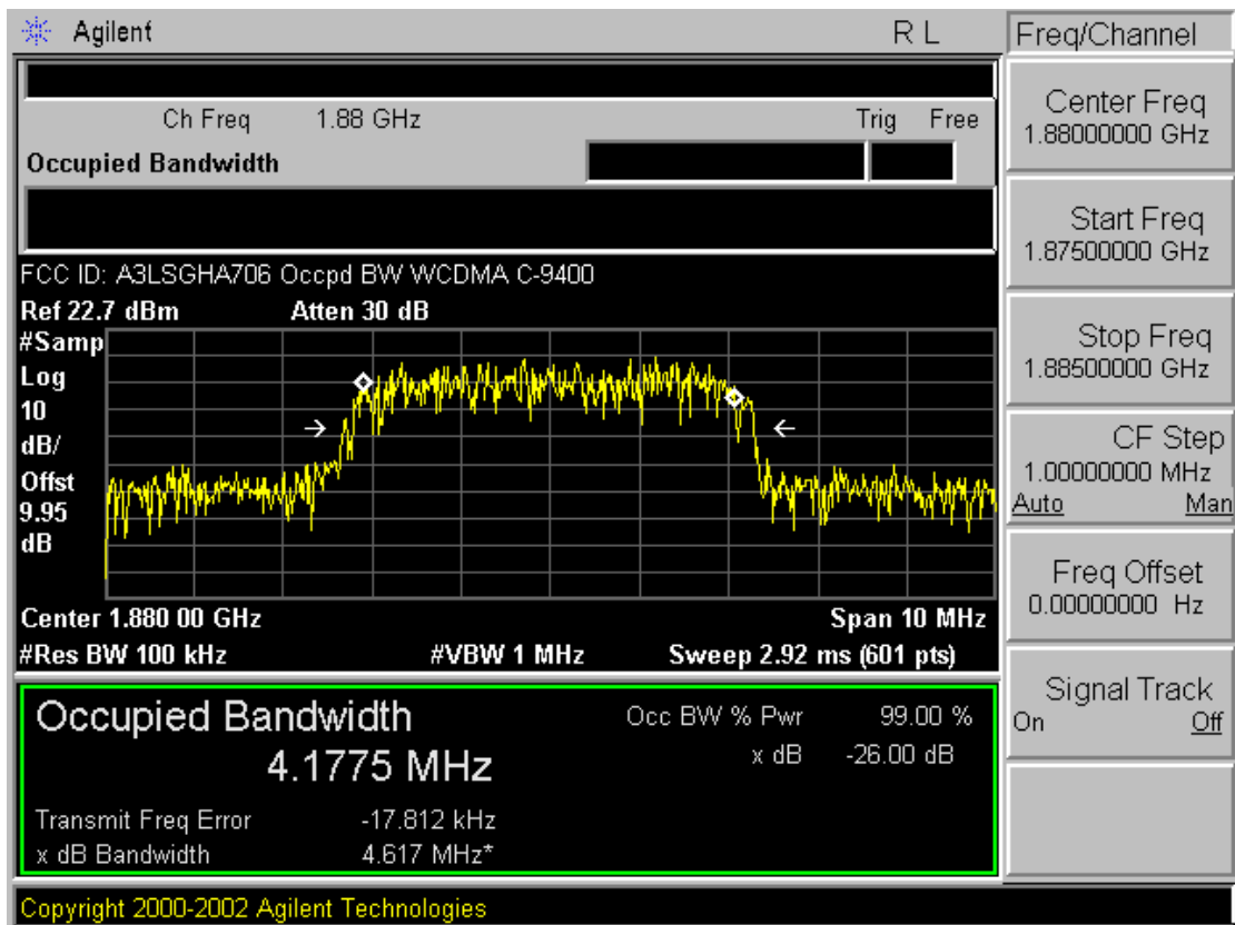
Plot A-18. Occupied Bandwidth Plot (PCS WCDMA Mode – Ch. 9400)
