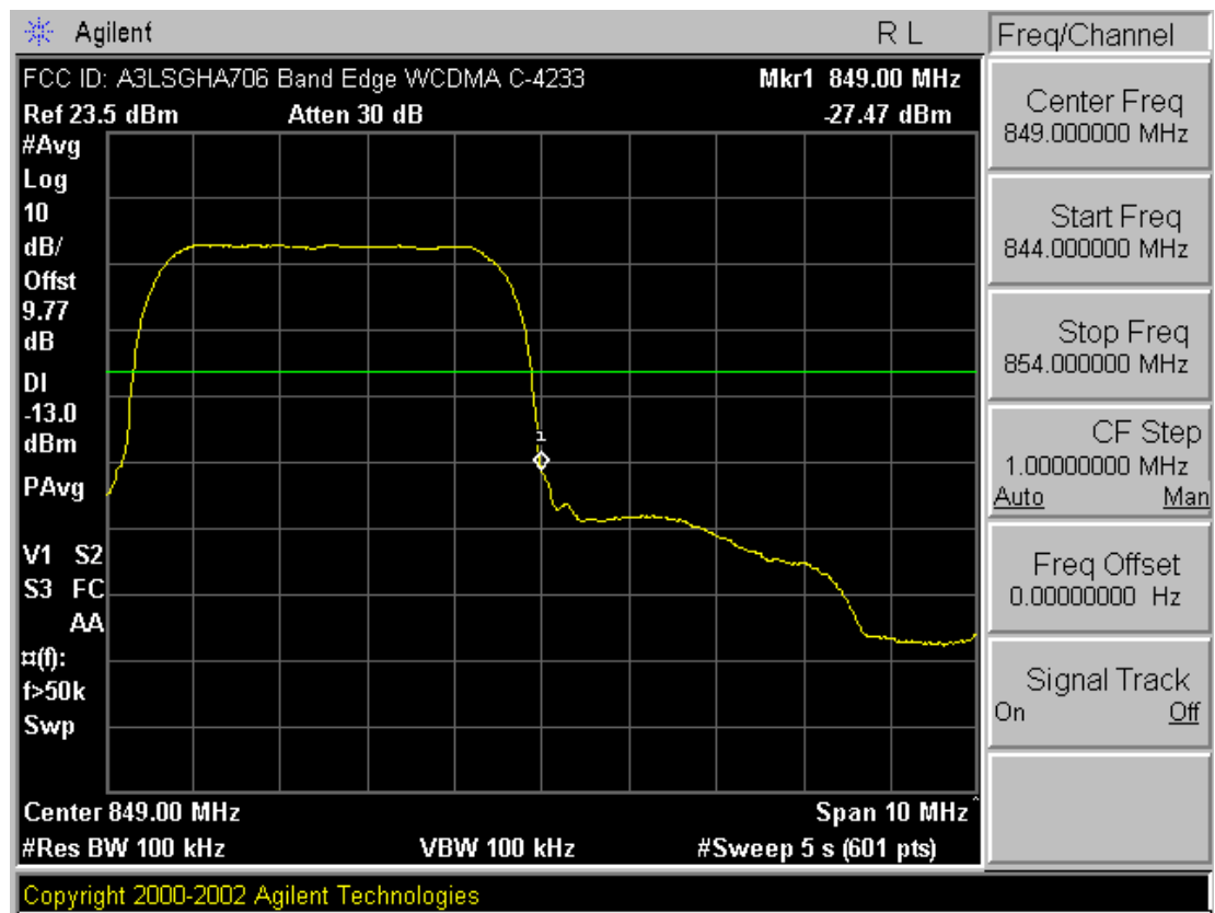
Plot A-10. Band Edge Plot (Cellular WCDMA Mode – Ch. 4233)
