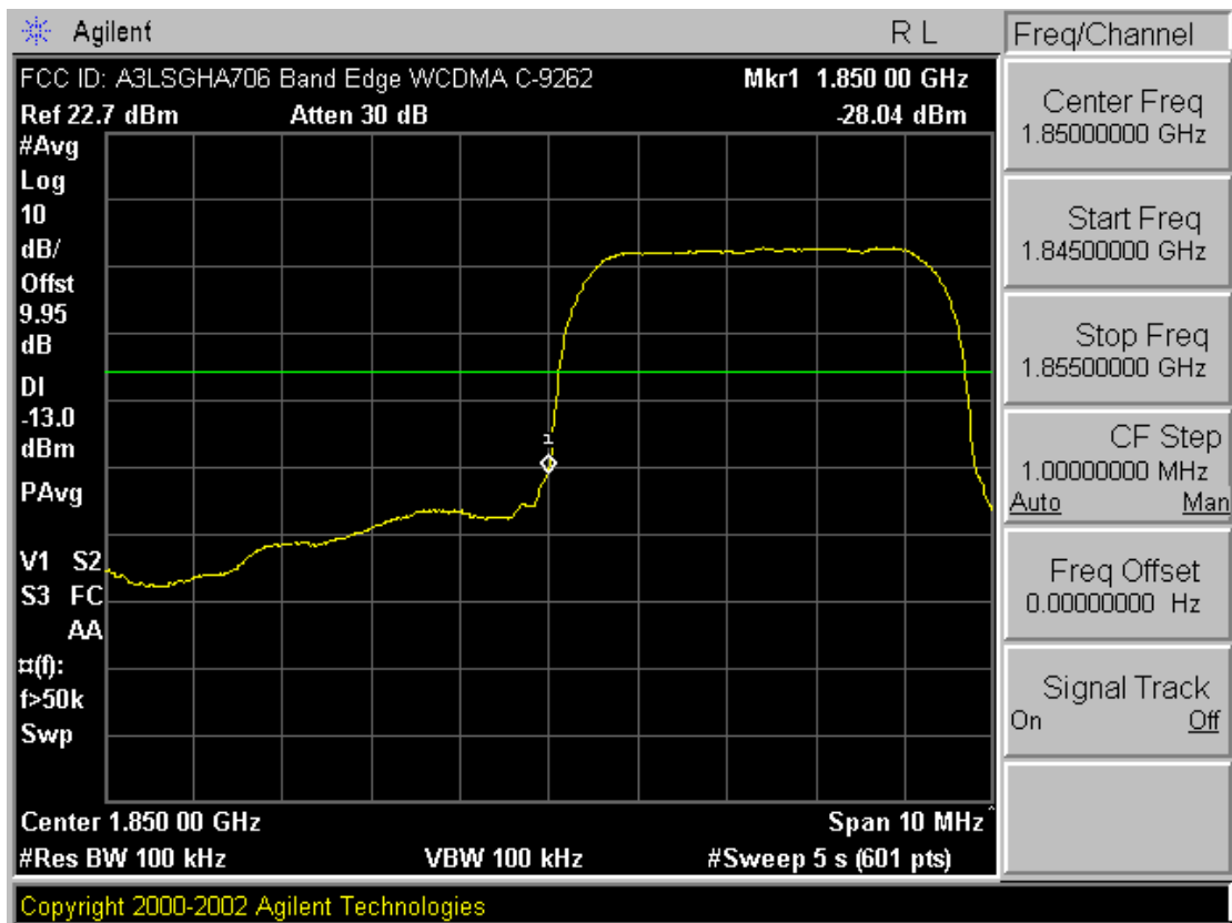
Plot A-14. Band Edge Plot (PCS WCDMA Mode – Ch. 9262)
