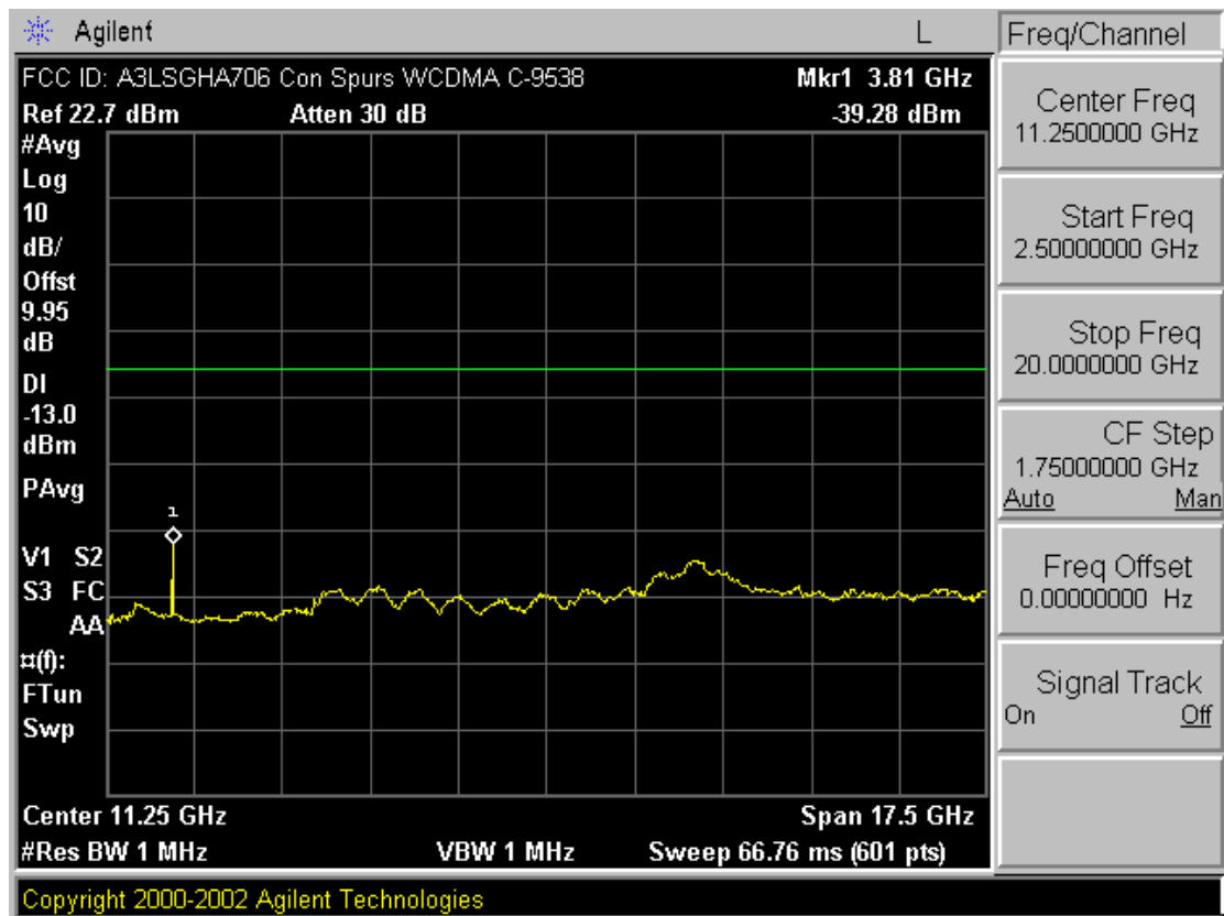
Plot A-20. Conducted Spurious Plot (PCS WCDMA Mode – Ch. 9538)
