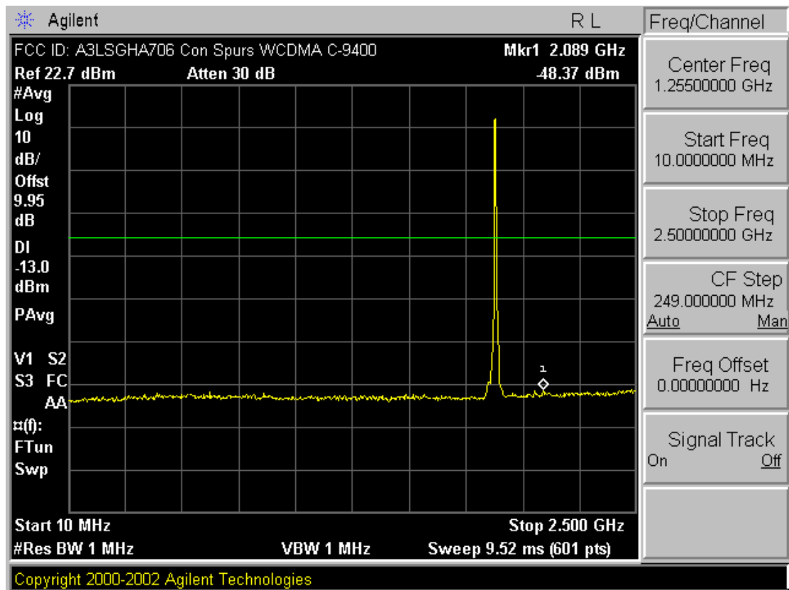
Plot A-16. Conducted Spurious Plot (PCS WCDMA Mode – Ch. 9400)
