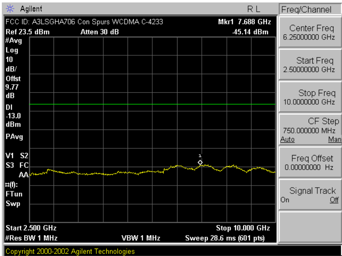
Plot A-9. Conducted Spurious Plot (Cellular WCDMA Mode – Ch. 4233)
