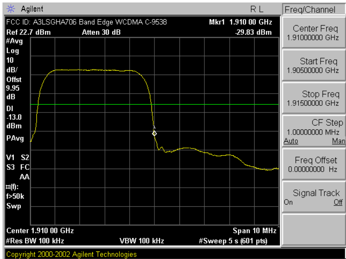
Plot A-21. Band Edge Plot (PCS WCDMA Mode – Ch. 9538)
