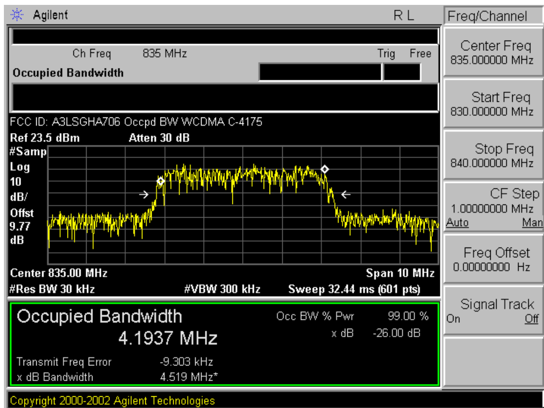
Plot A-7. Occupied Bandwidth Plot (Cellular WCDMA Mode – Ch. 4175)
