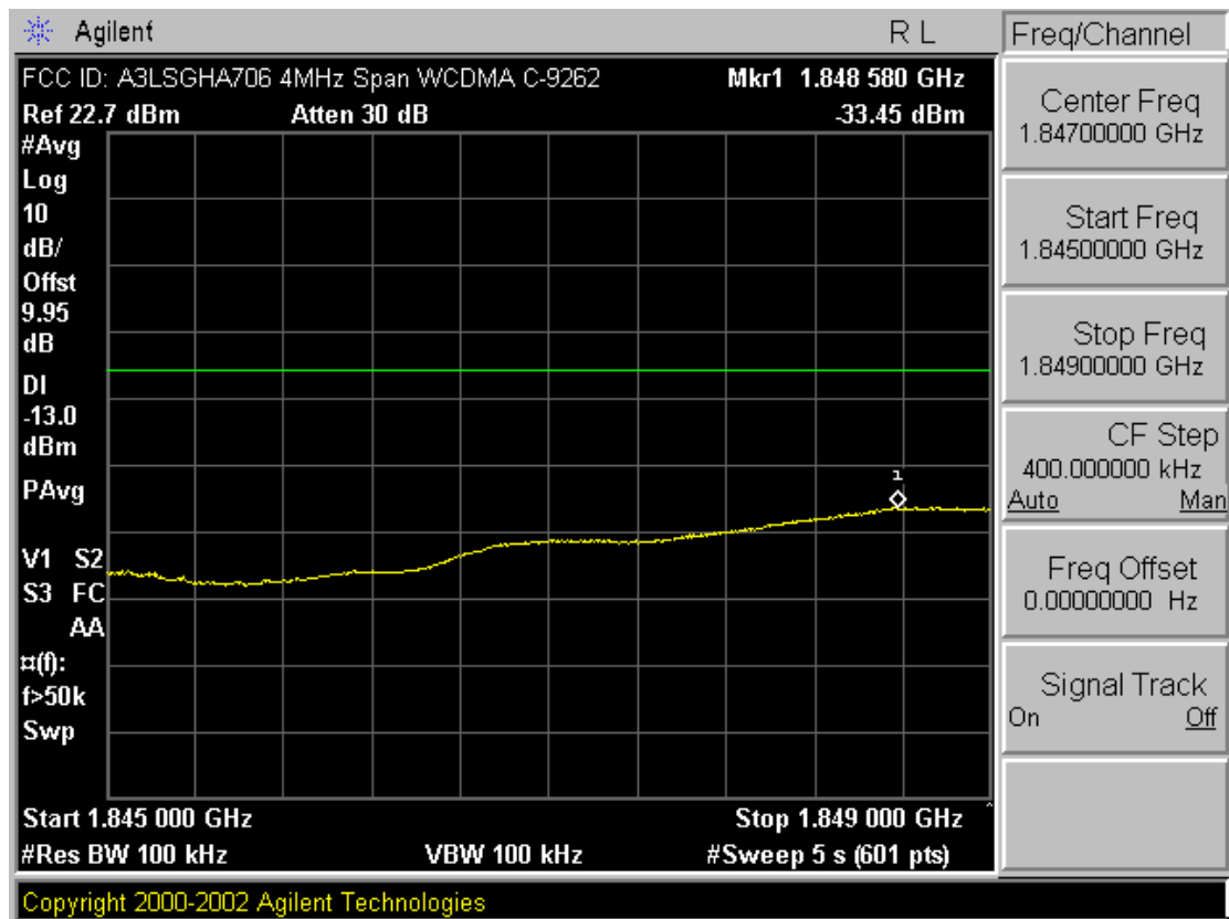
Plot A-15. 4MHz Span Plot (PCS WCDMA Mode – Ch. 9262)
