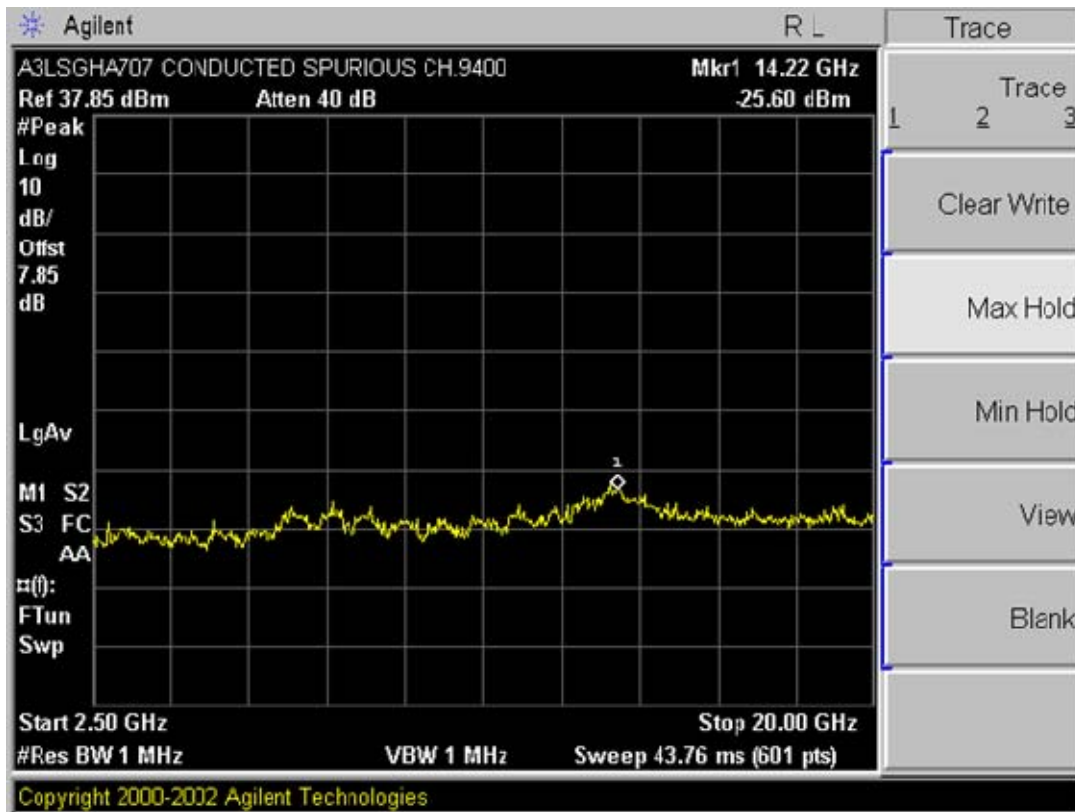
Plot A-14. Conducted Spurious Plot (PCS WCDMA Mode – Ch. 9400)
