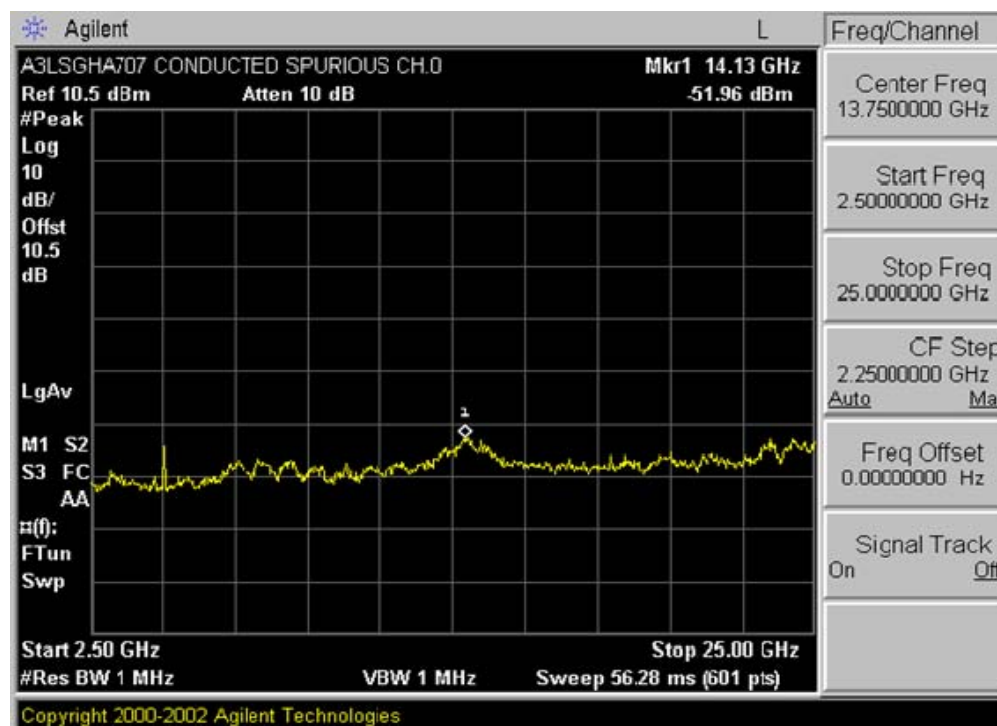
Plot 6-11. Conducted Spurious Plot (Bluetooth – Ch. 0)
