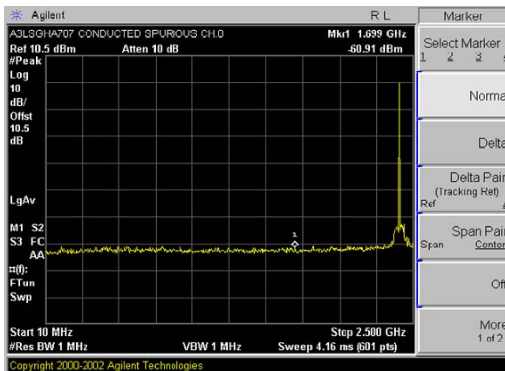
Plot 6-10. Conducted Spurious Plot (Bluetooth – Ch. 0)
