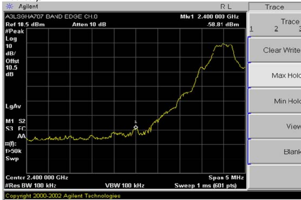
Plot 6-4. Band Edge Plot (Bluetooth – Ch. 0)
