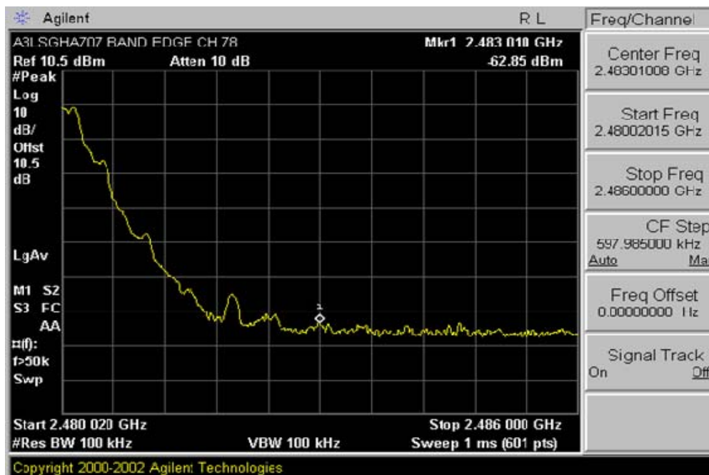
Plot 6-5. Band Edge Plot (Bluetooth – Ch. 78)
