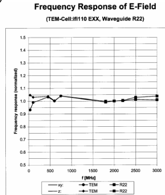
Figure 4 E-Field Probe Frequency Response
