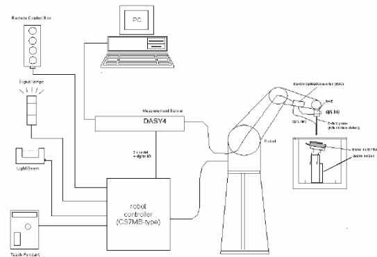
Figure 7 SPEAG Robotic System Diagram
