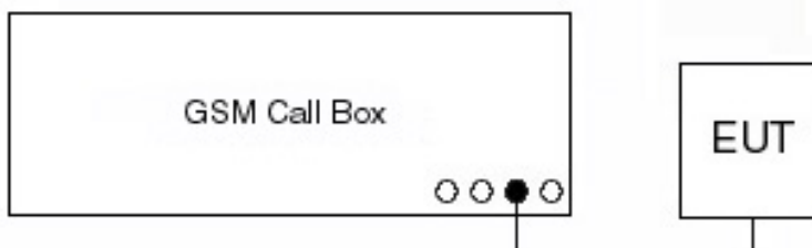
Figure 6-1. GSM Conducted Power Test Setup Diagram
