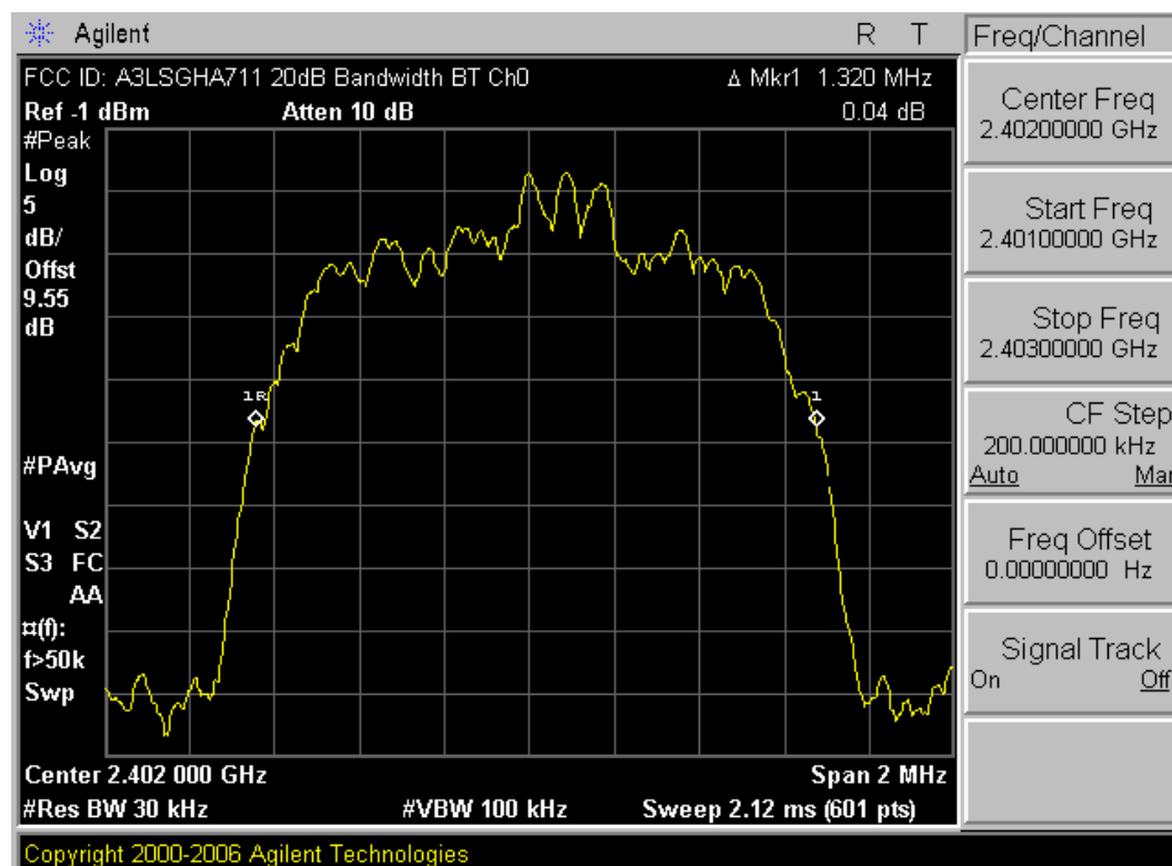
Plot 6-1. 20dB Bandwidth Plot (Bluetooth 2.0 + EDR – Ch. 0)
