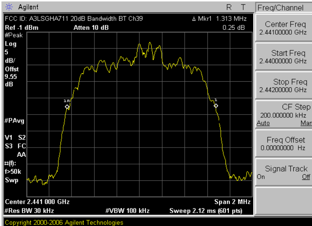
Plot 6-2. 20dB Bandwidth Plot (Bluetooth 2.0 + EDR – Ch. 39)
