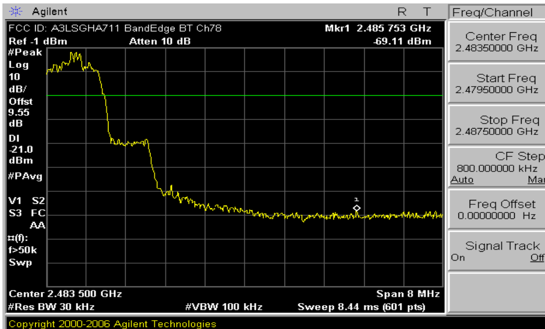
Plot 6-5. Band Edge Plot (Bluetooth 2.0 + EDR – Ch. 78)
