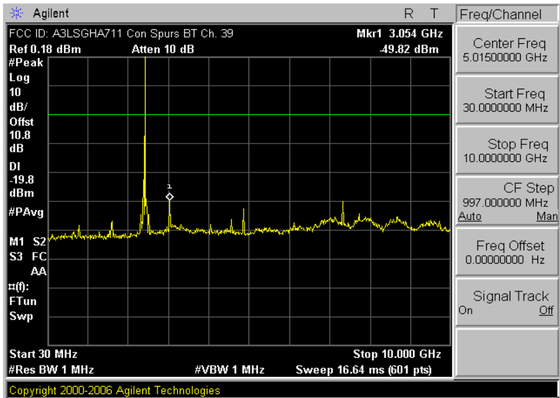
Plot 6-12. Conducted Spurious Plot (Bluetooth – Ch. 39)
