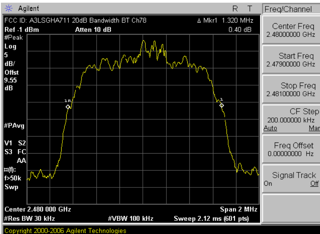
Plot 6-3. 20dB Bandwidth Plot (Bluetooth 2.0 + EDR – Ch. 78)
