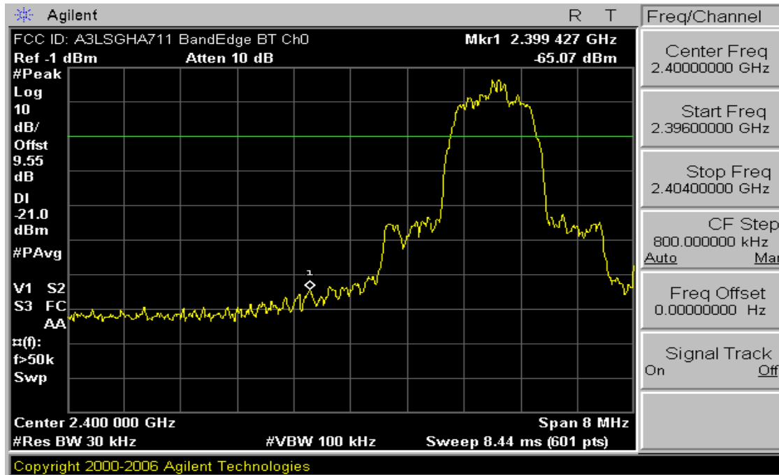
Plot 6-4. Band Edge Plot (Bluetooth 2.0 + EDR – Ch. 0)
