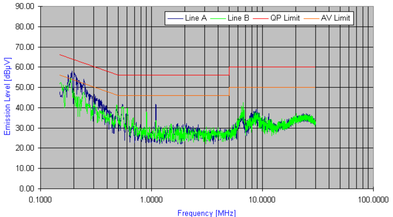
Plot 7-1. Line-Conducted Test Plot
