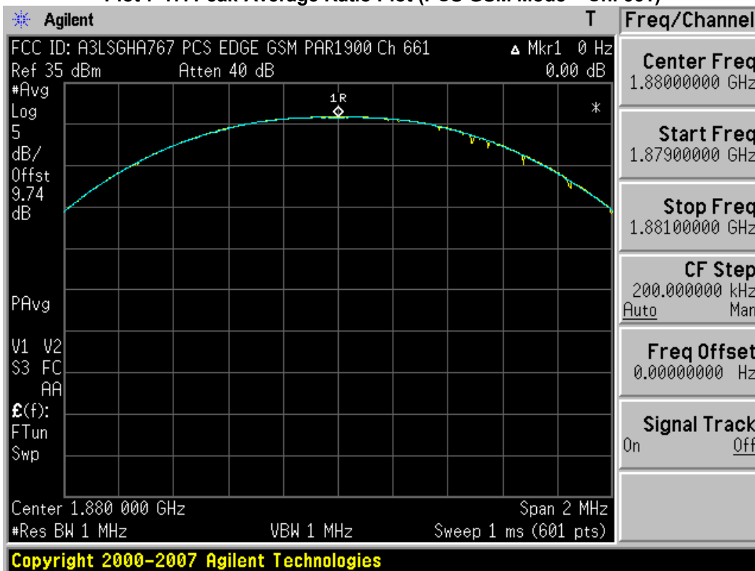
Plot 7-18. Peak-Average Ratio Plot (PCS EDGE Mode – Ch. 661)
