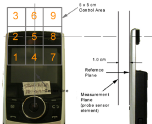
Figure 17-3 5x5 Scan grid above WD
