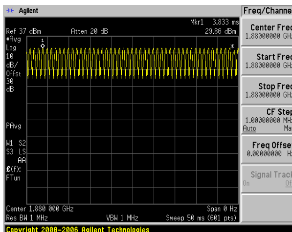
Figure 8.5 GSM1900 80% AM Signal
