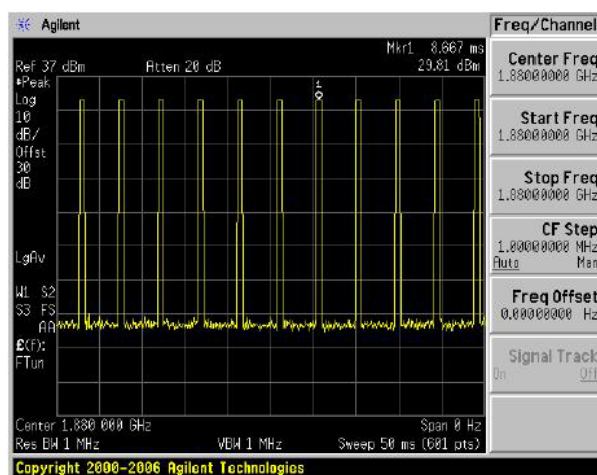
Figure 8.3 GSM1900 Signal
