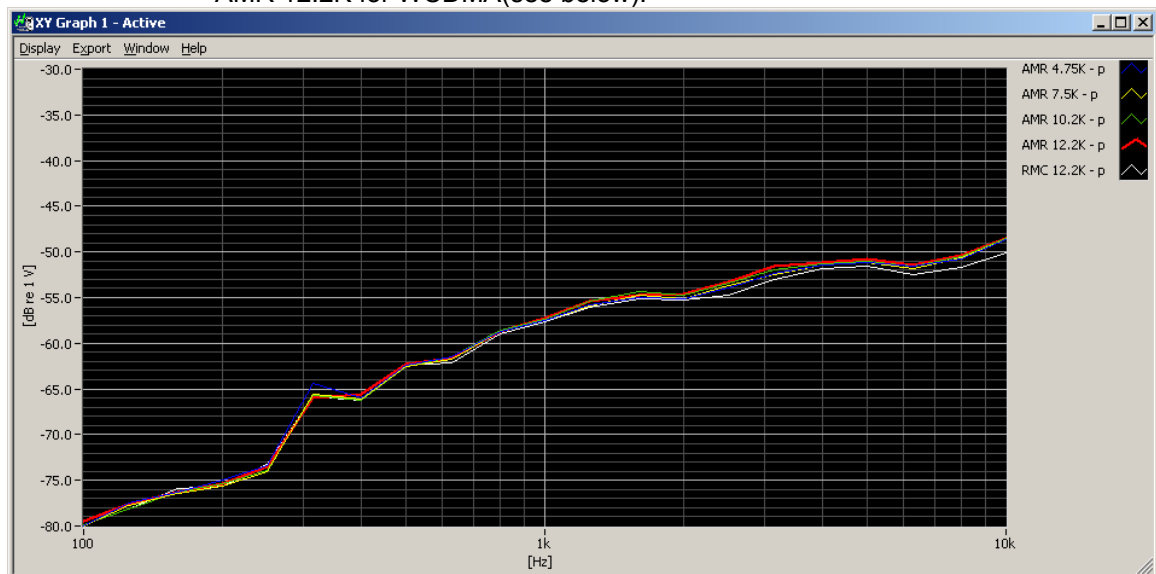
Figure 5-9 Vocoder Analysis for ABM Noise(WCDMA)
