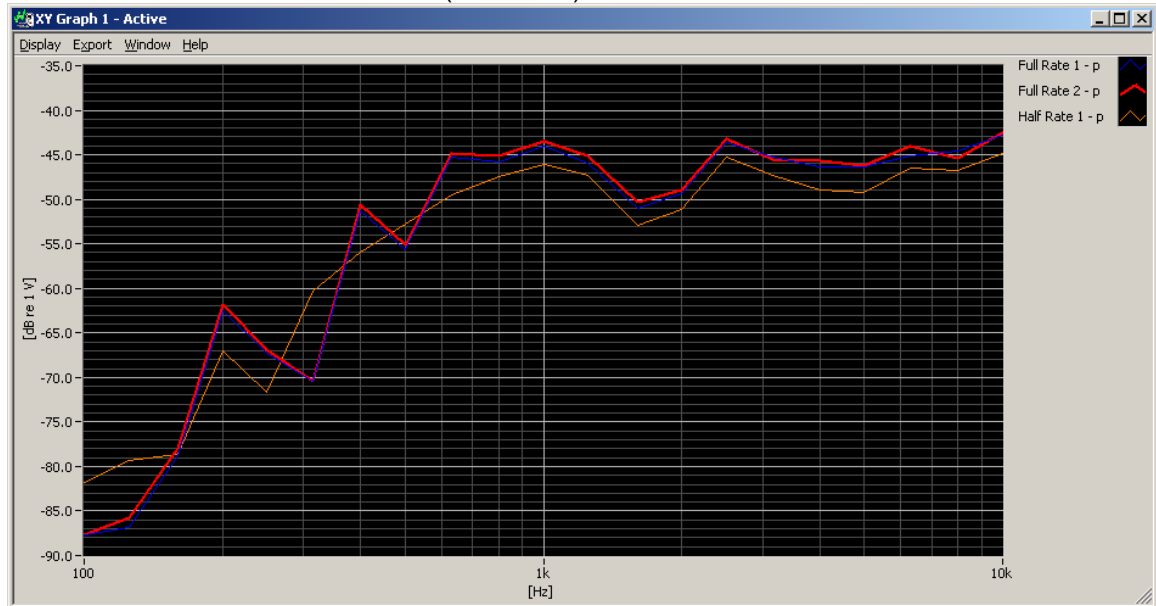
Figure 5-8 Vocoder Analysis for ABM Noise(GSM)
