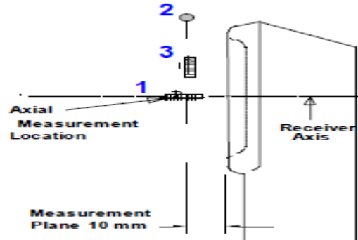
Figure 5-6 Measurement Distance
