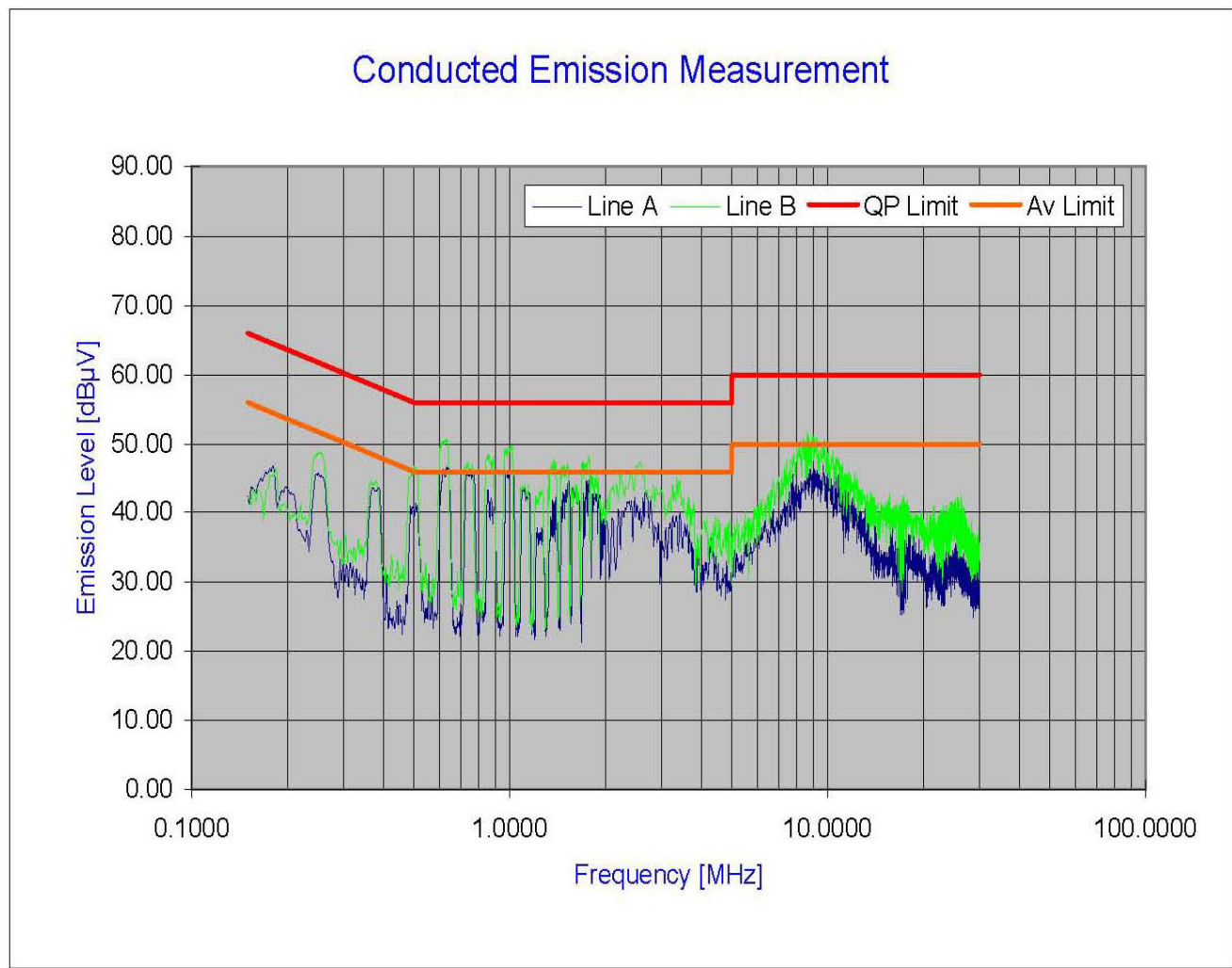
Plot 6-18. Line Conducted Plot with Bluetooth
