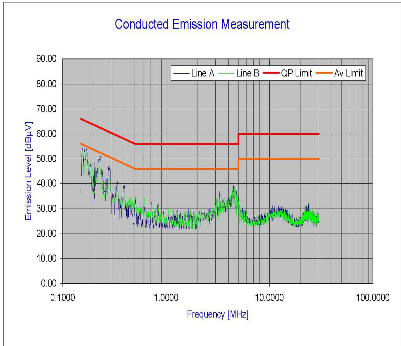
Plot 7-1. Line-Conducted Test Plot
