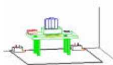
Figure 3-2. Line Conducted Emission Test Set-Up
