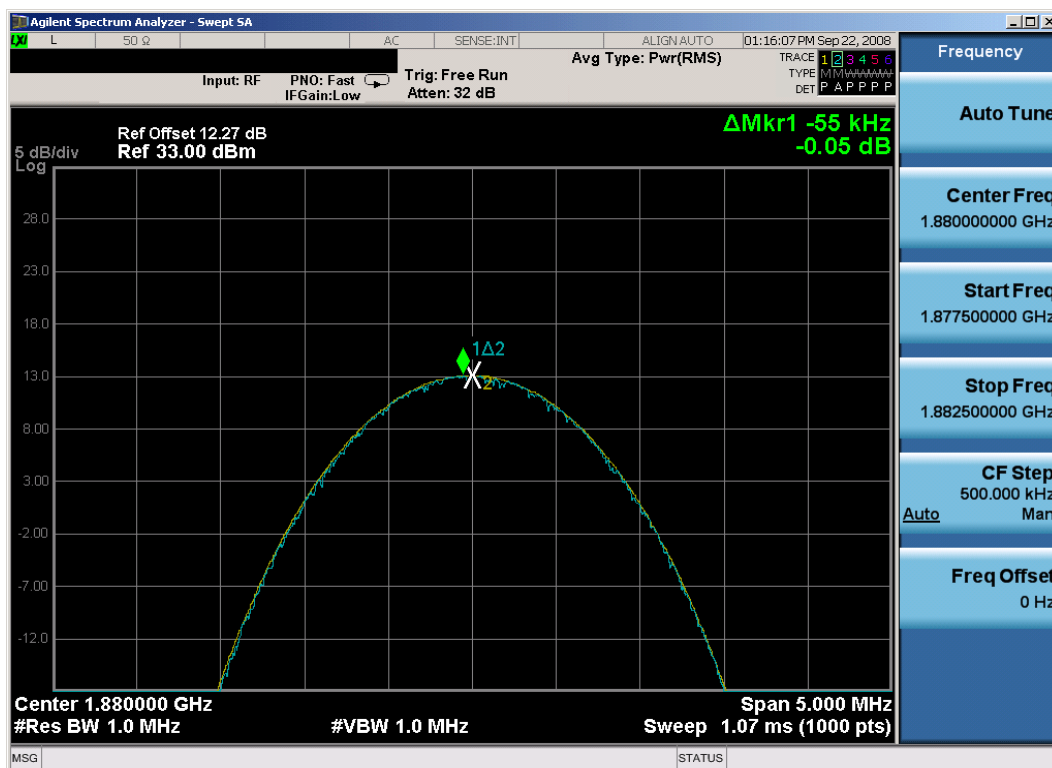
Plot 7-18. Peak-Average Ratio Plot (EDGE1900 Mode – Ch. 661)
