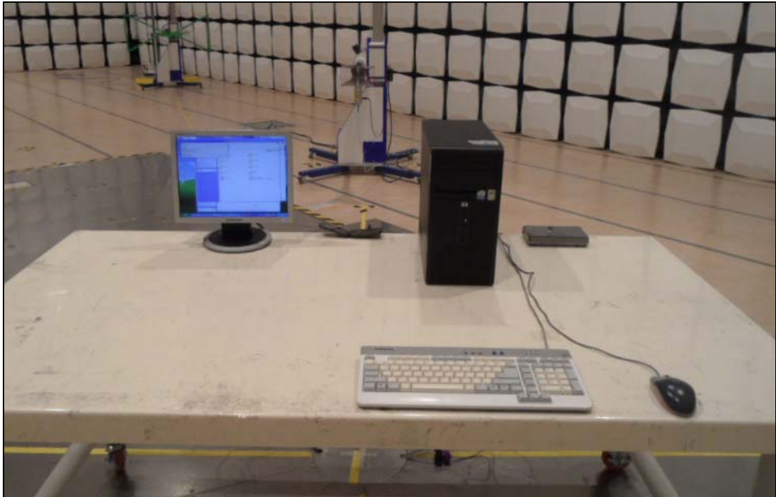
[ Radiated Disturbance for Above 1 GHz – Front ]
