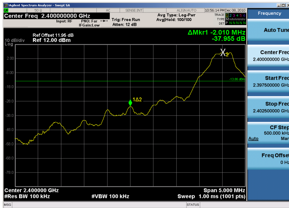
Plot 6-10. Band Edge Plot (Bluetooth, 1Mbps – Ch. 0)
