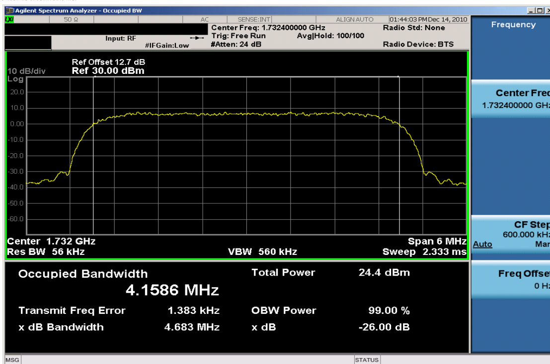
Plot 7-29. Occupied Bandwidth Plot (AWS WCDMA Mode – Ch. 1412)
