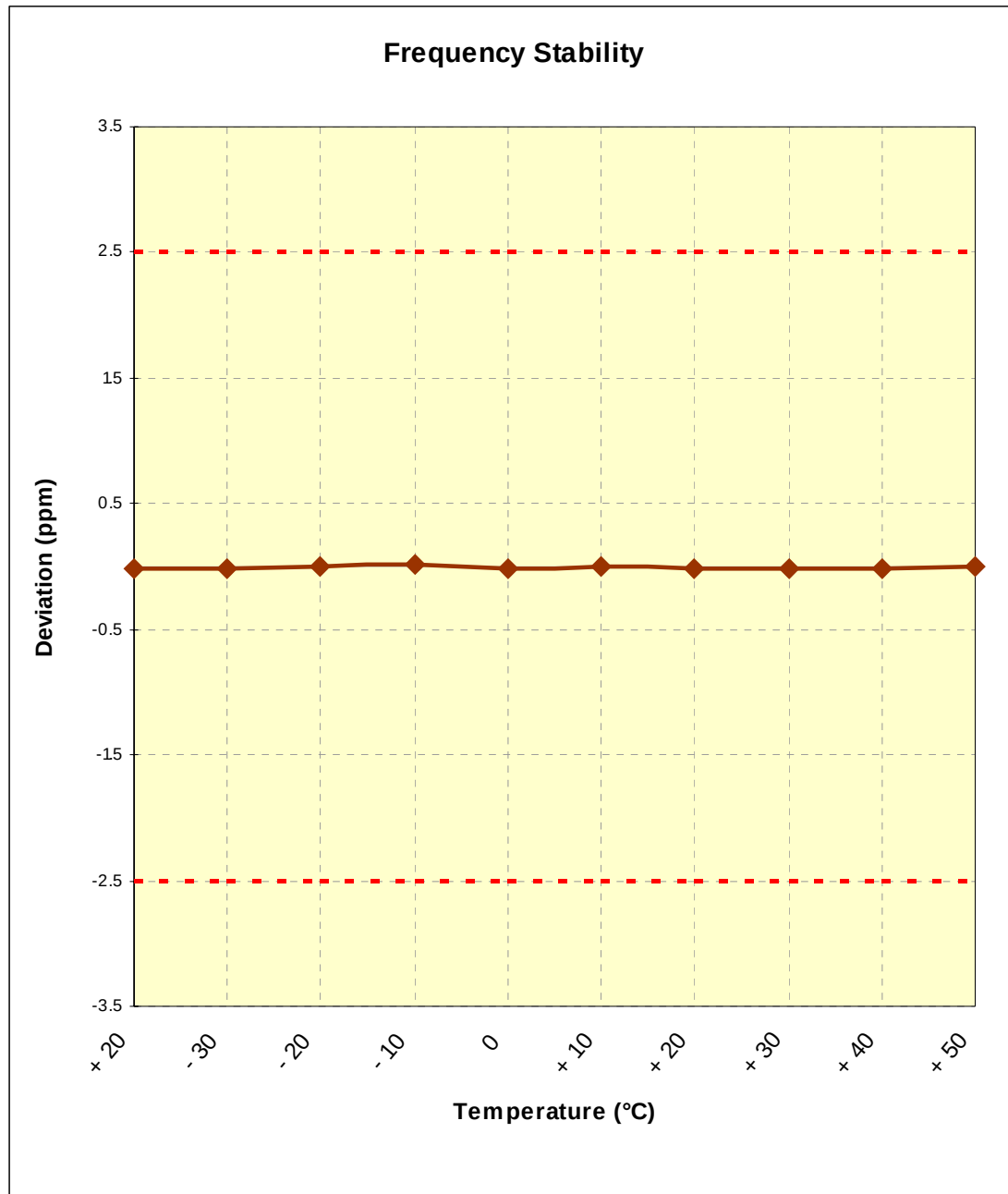
Figure 6-3. Frequency Stability Graph (AWS WCDMA Mode – Ch. 1412)
