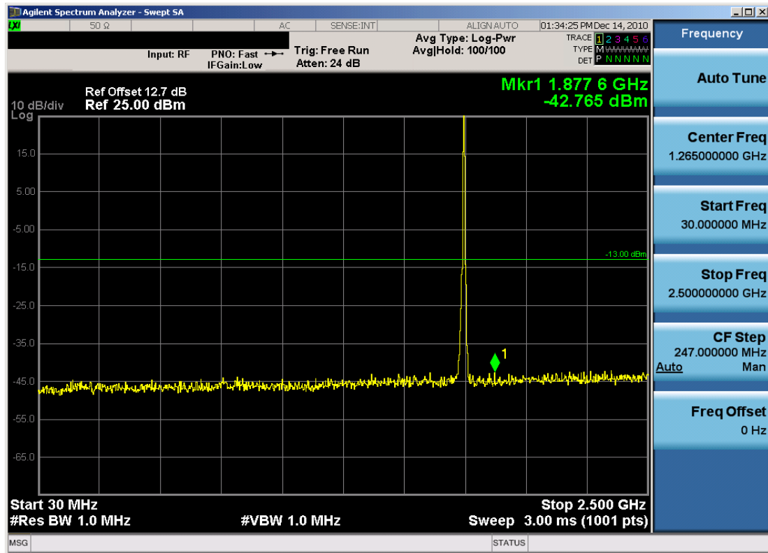
Plot 7-31. Conducted Spurious Plot (AWS WCDMA Mode – Ch. 1862)
