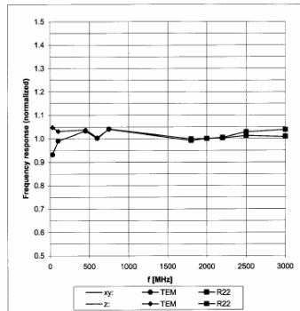
Figure 5-5 E-Field Probe Frequency Response
