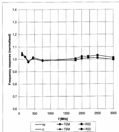
Figure 5-6 H-Field Probe Frequency Response
