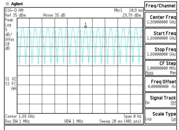
Figure 8-3 80% AM Signal
