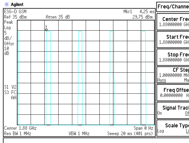
Figure 8-4 GSM Signal
