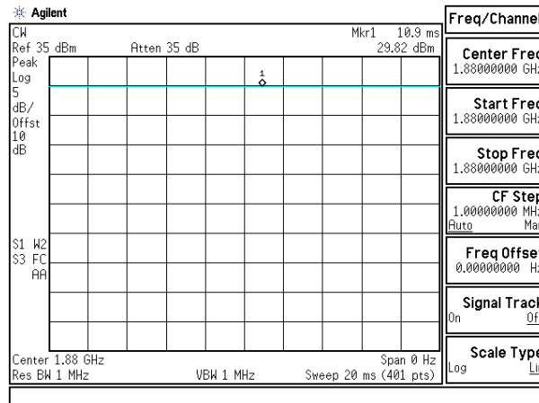
Figure 8-2 CW Signal
