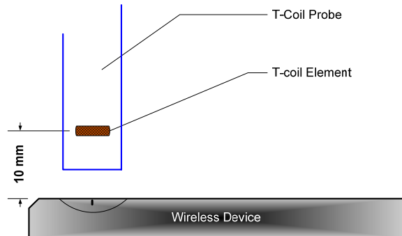
Figure 5-11 Measurement Distance
