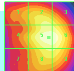
Cellular E-field – Max 218.9 V/m (M3)
