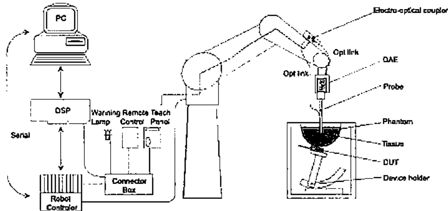
Figure 3.1 SAR Measurement System Setup
