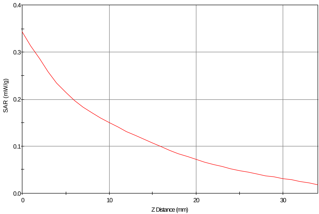
SAR - Z Axis at Hotspot x:48.0 y:3.0
