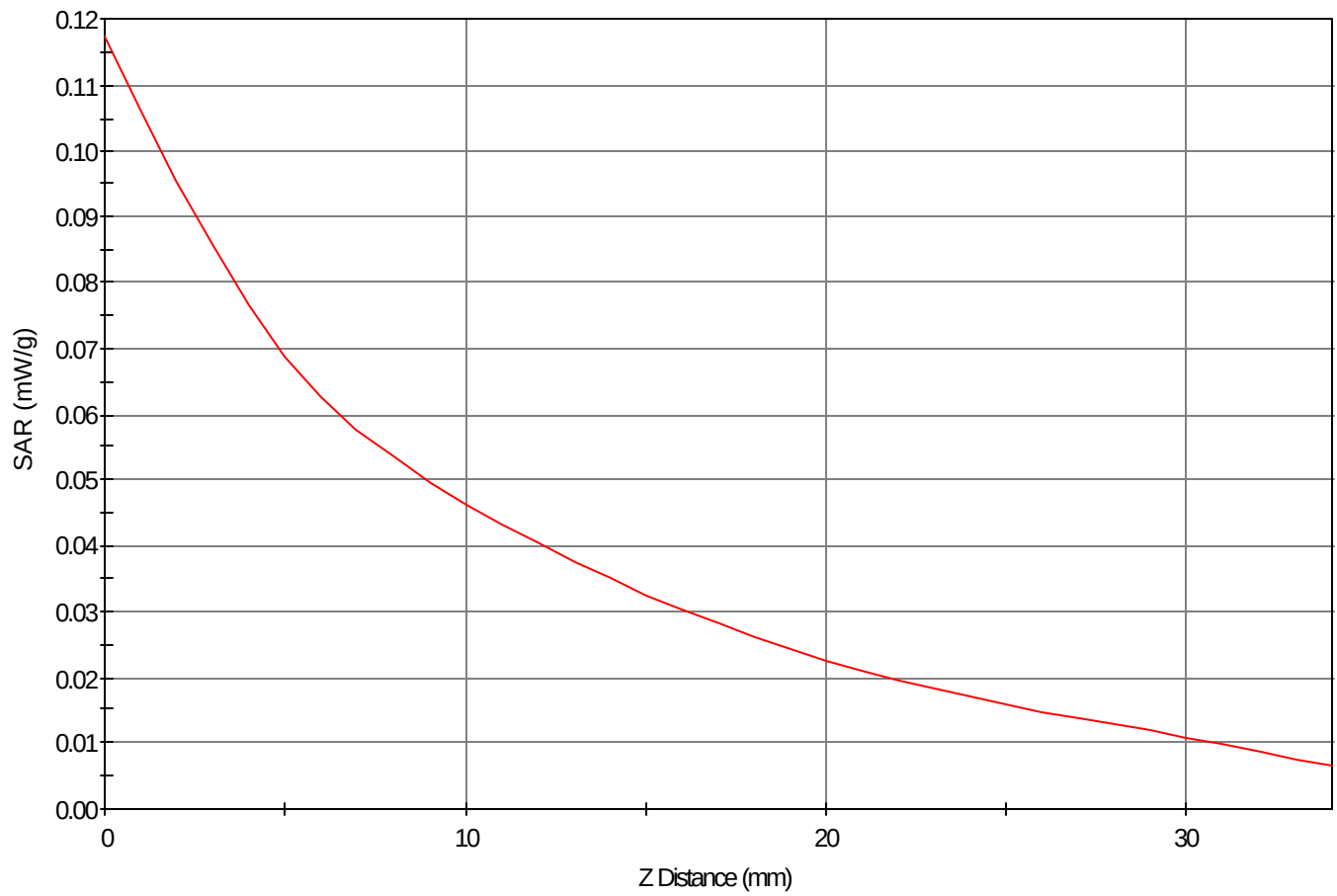
SAR - Z Axis at Hotspot x:55.0 y:10.0
