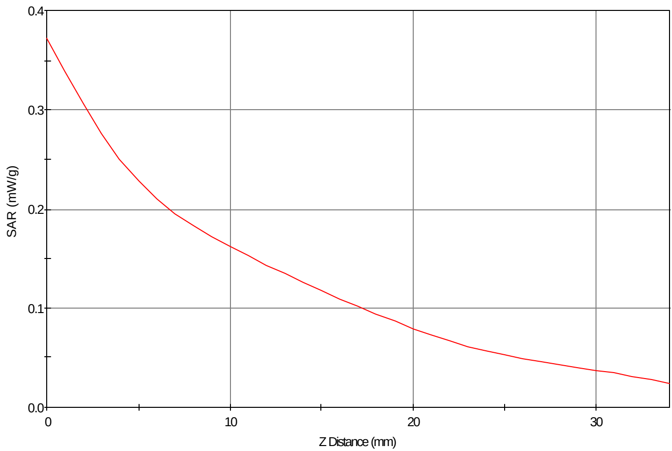
SAR - Z Axis at Hotspot x:37.0 y:-4.0
