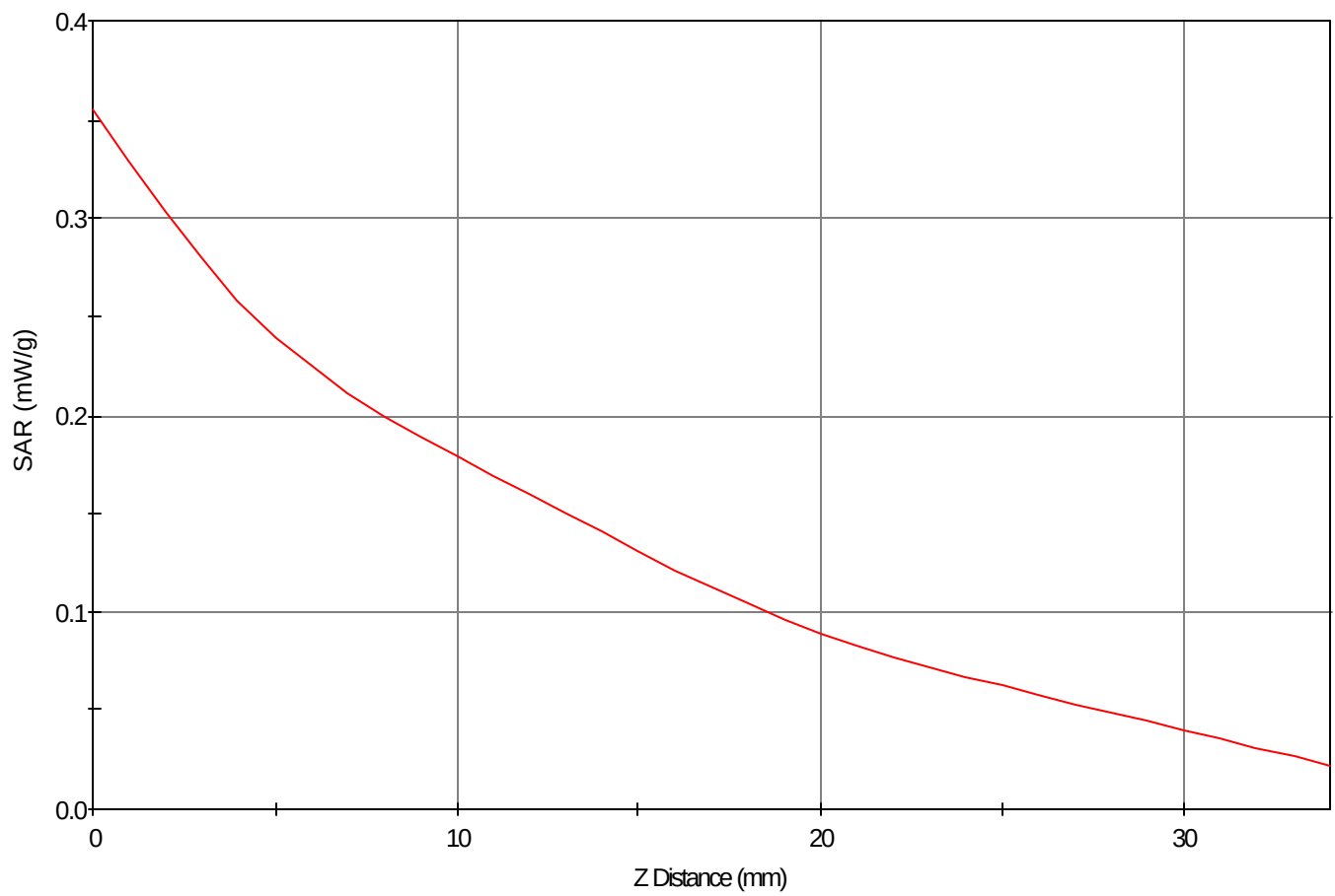
SAR - Z Axis at Hotspot x:37.0 y:1.0
