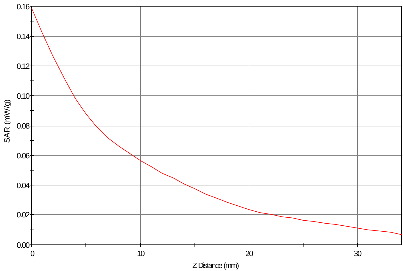
SAR - Z Axis at Hotspot x:58.0 y:10.0
