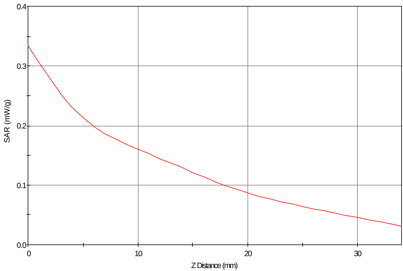
SAR - Z Axis at Hotspot x:36.0 y:7.0
