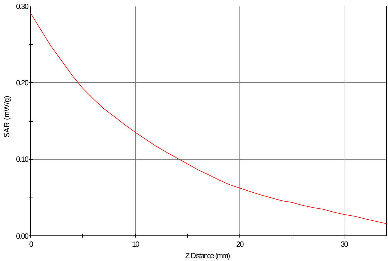
SAR - Z Axis at Hotspot x:44.0 y:-2.0
