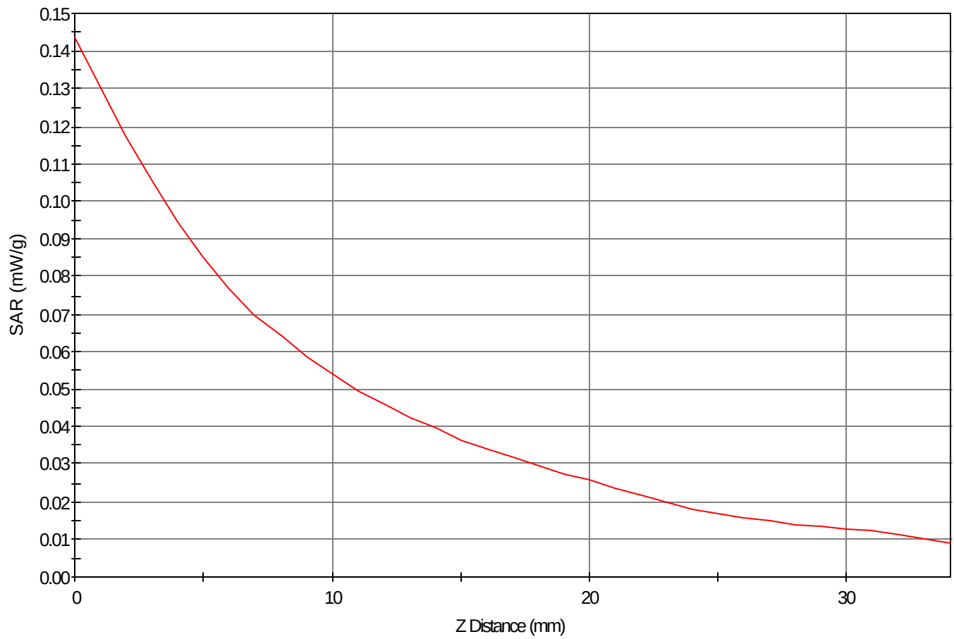
SAR - Z Axis at Hotspot x:61.0 y:11.0
