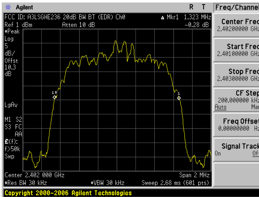
Plot 6-1. 20dB Bandwidth Plot (Bluetooth 2.0 with Enhanced Data Rate – Ch. 0)
