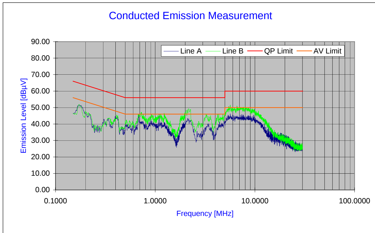
Plot 6-16. Line Conducted Plot with Bluetooth
