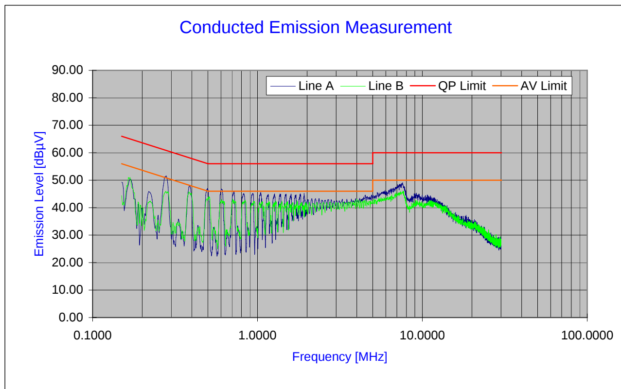
Plot 7-1. Line-Conducted Test Plot
