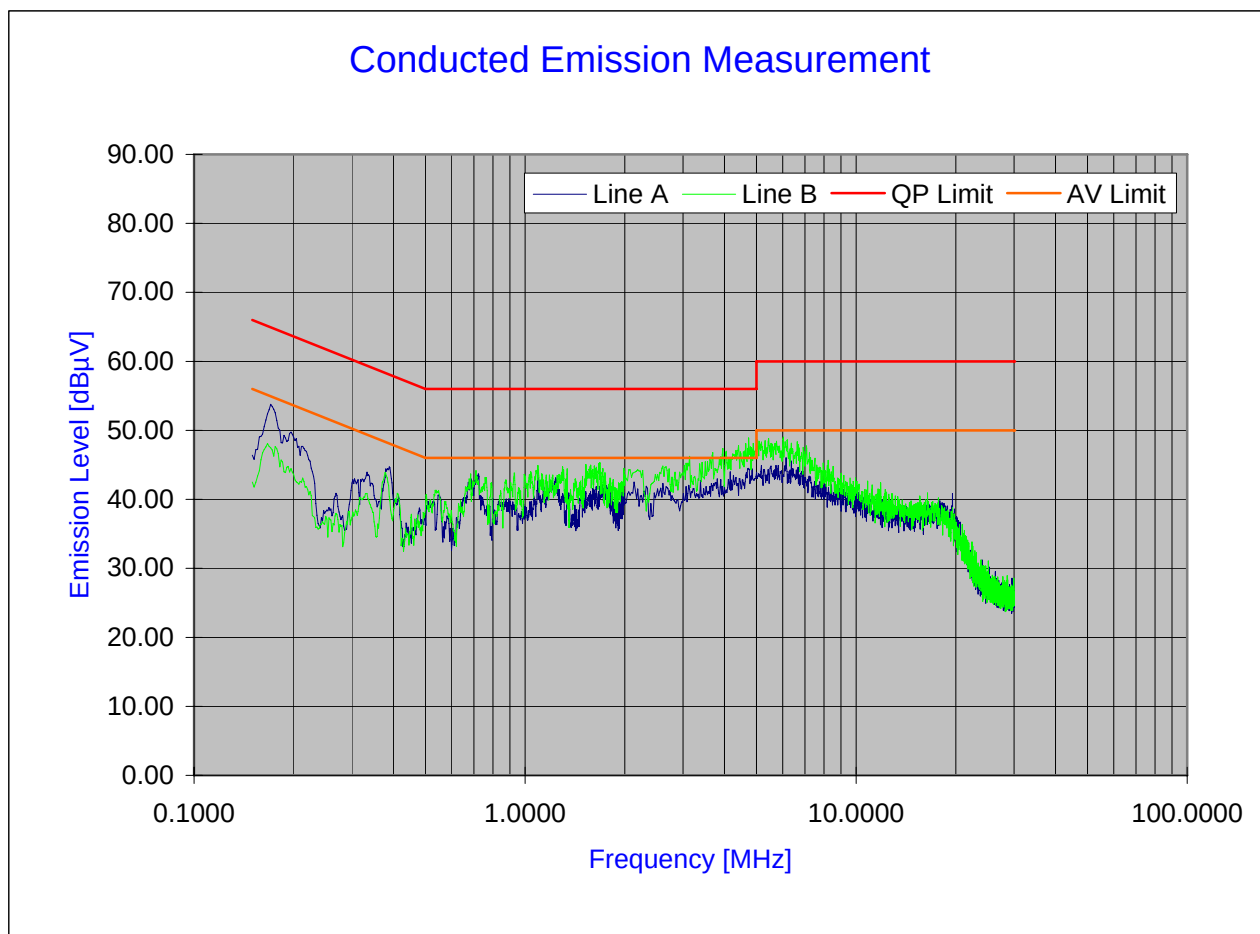
Plot 1. Line Conducted Plot with Bluetooth
