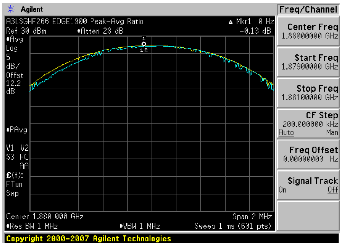
Plot 7-22. Peak-Average Ratio (EDGE1900 Mode – Ch. 661)
