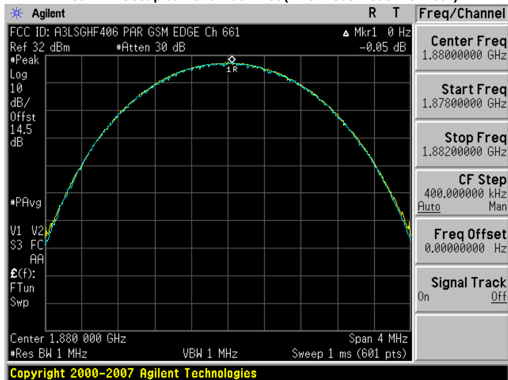
Plot 7-22. Peak to Average Ratio (EDGE1900 Mode - Ch. 661)
