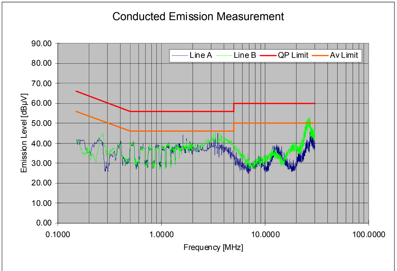
Plot 7-1. Line-Conducted Test Plot
