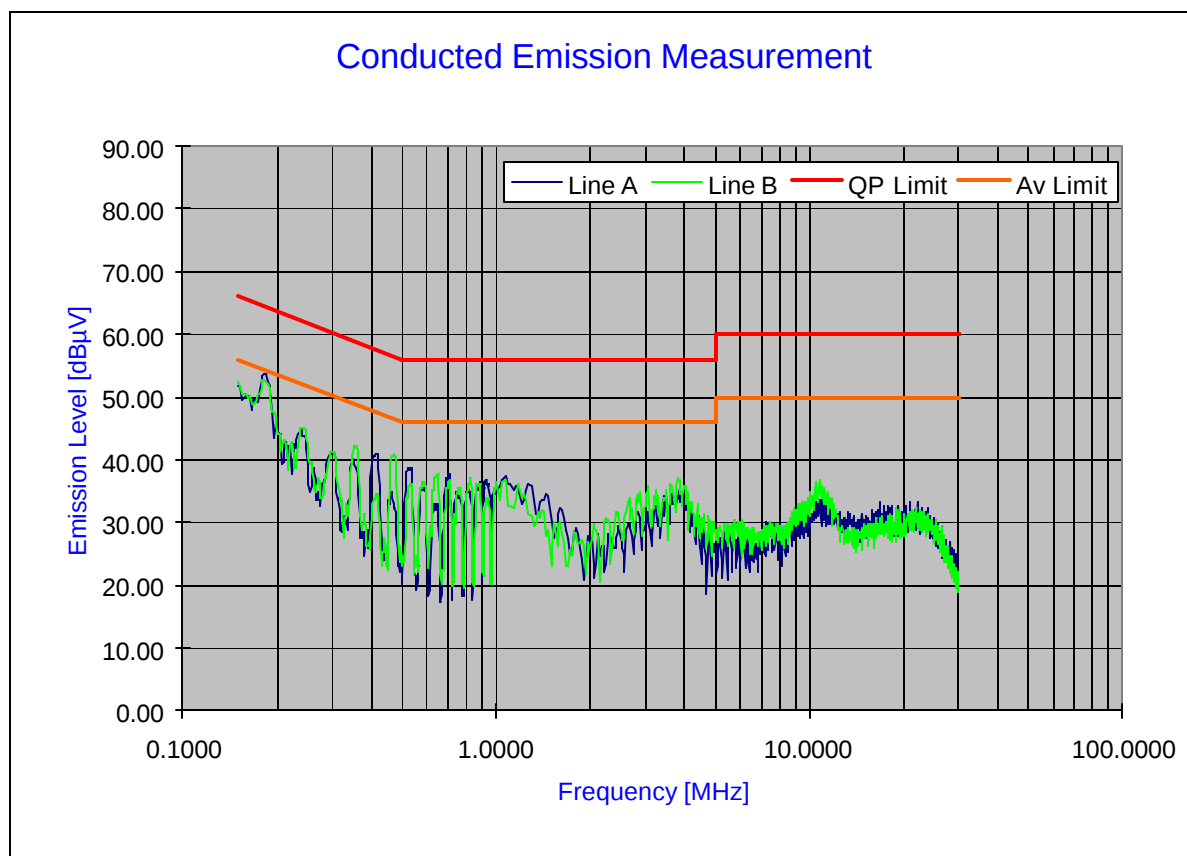
Plot 7-1. Line-Conducted Test Plot
