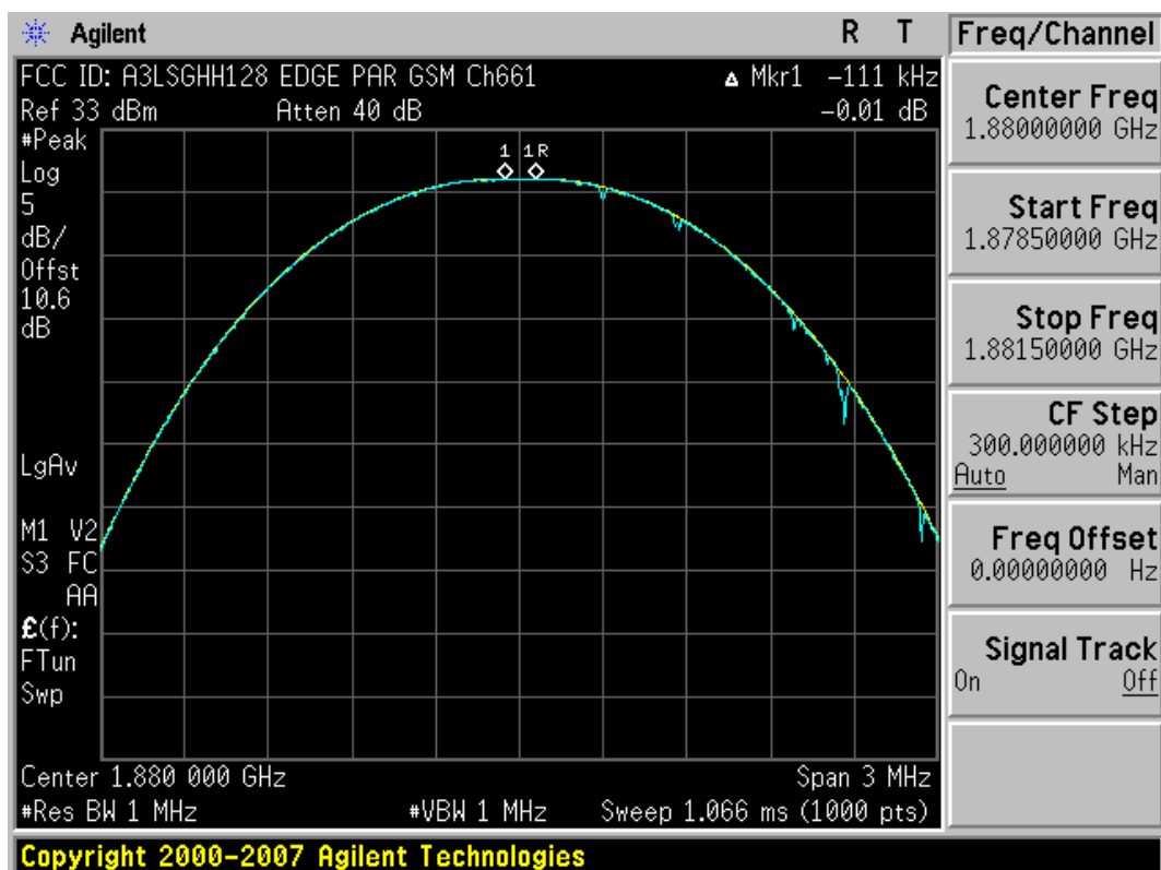
Plot 7-12. Peak to Average Ratio Plot (EDGE1900 Mode – Ch. 661)
