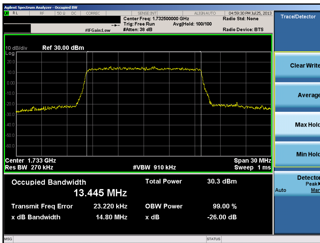
Plot 9-25. Occupied Bandwidth Plot (15.0MHz QPSK – RB Size 75)
