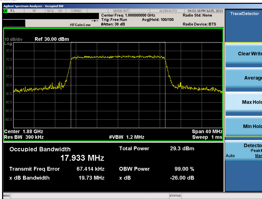
Plot 10-34. Occupied Bandwidth Plot (20.0MHz 16-QAM – RB Size 100)
