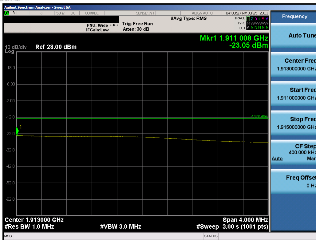
Plot 10-28. Upper Extended Band Edge Plot (15.0MHz QPSK – RB Size 75)
