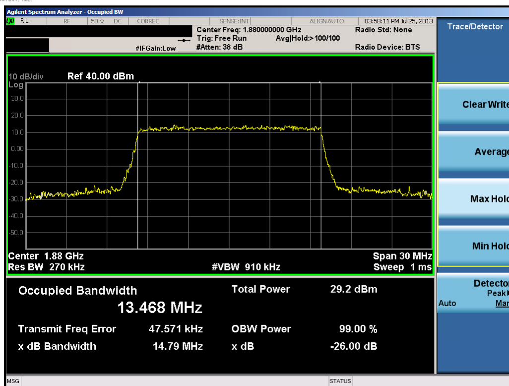
Plot 10-26. Occupied Bandwidth Plot (15.0MHz 16-QAM – RB Size 75)
