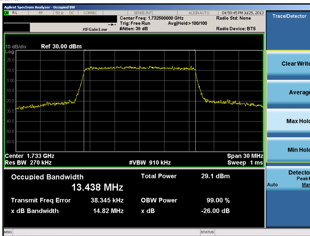
Plot 9-26. Occupied Bandwidth Plot (15.0MHz 16-QAM – RB Size 75)
