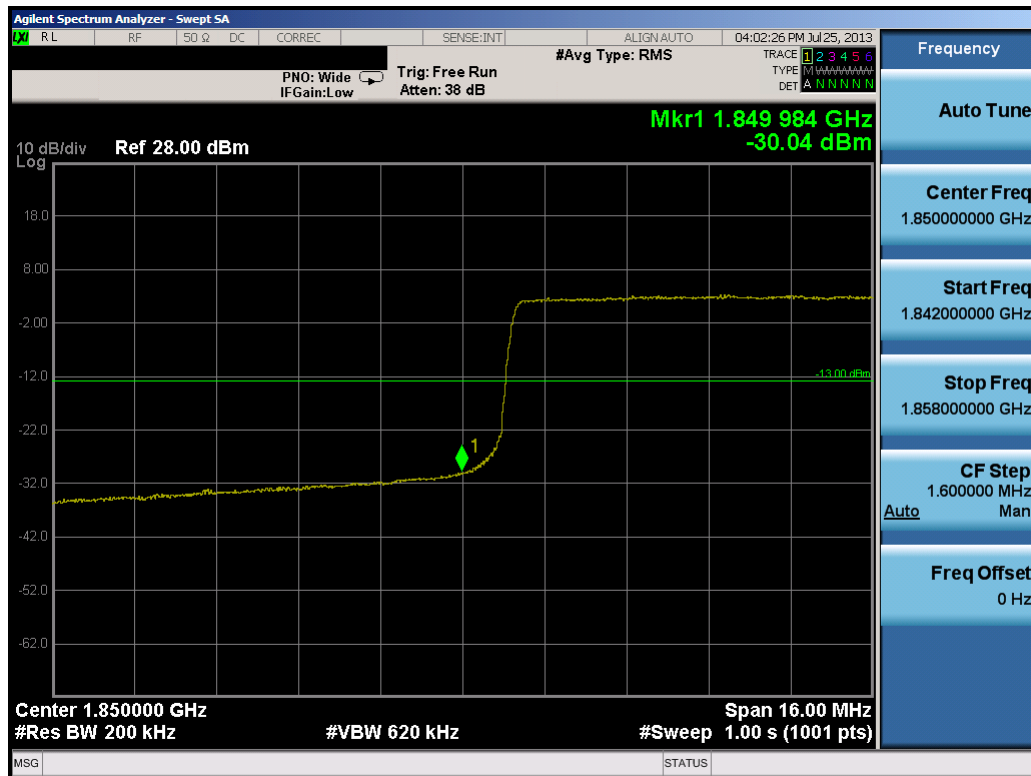
Plot 10-31. Lower Band Edge Plot (20.0MHz QPSK – RB Size 100)
