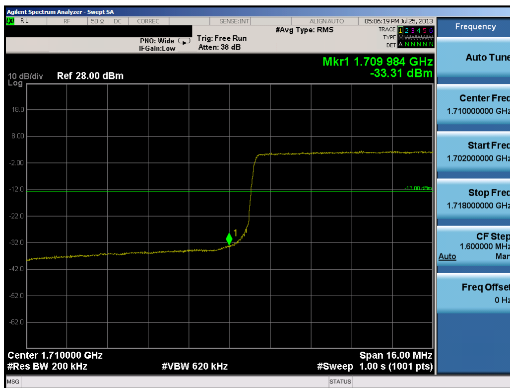
Plot 9-31. Lower Band Edge Plot (20.0MHz QPSK – RB Size 100)
