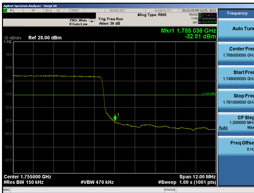
Plot 9-27. Upper Band Edge Plot (15.0MHz QPSK – RB Size 75)
