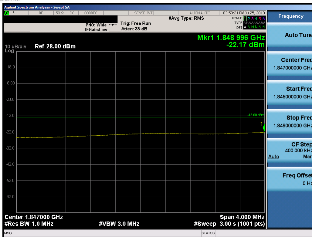
Plot 10-24. Lower Extended Band Edge Plot (15.0MHz QPSK – RB Size 75)
