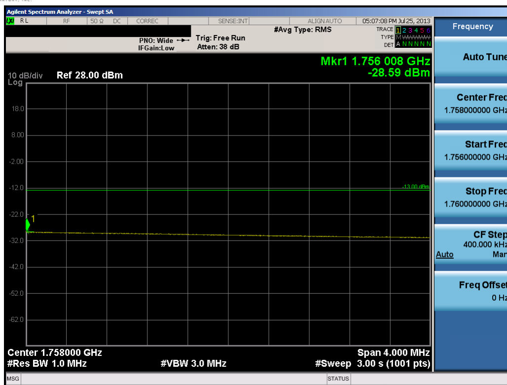
Plot 9-36. Upper Extended Band Edge Plot (20.0MHz QPSK – RB Size 100)
