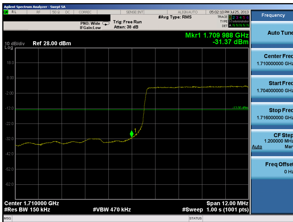
Plot 9-23. Lower Band Edge Plot (15.0MHz QPSK – RB Size 75)
