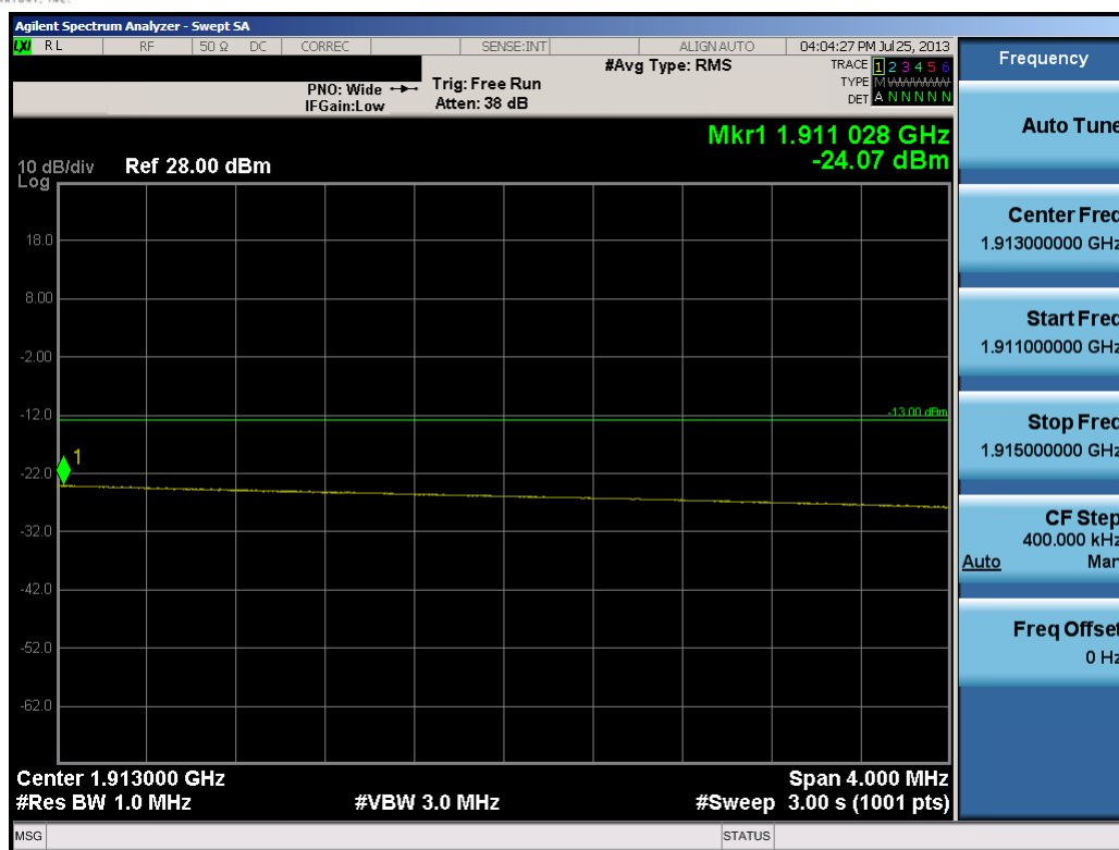
Plot 10-36. Upper Extended Band Edge Plot (20.0MHz QPSK – RB Size 100)
