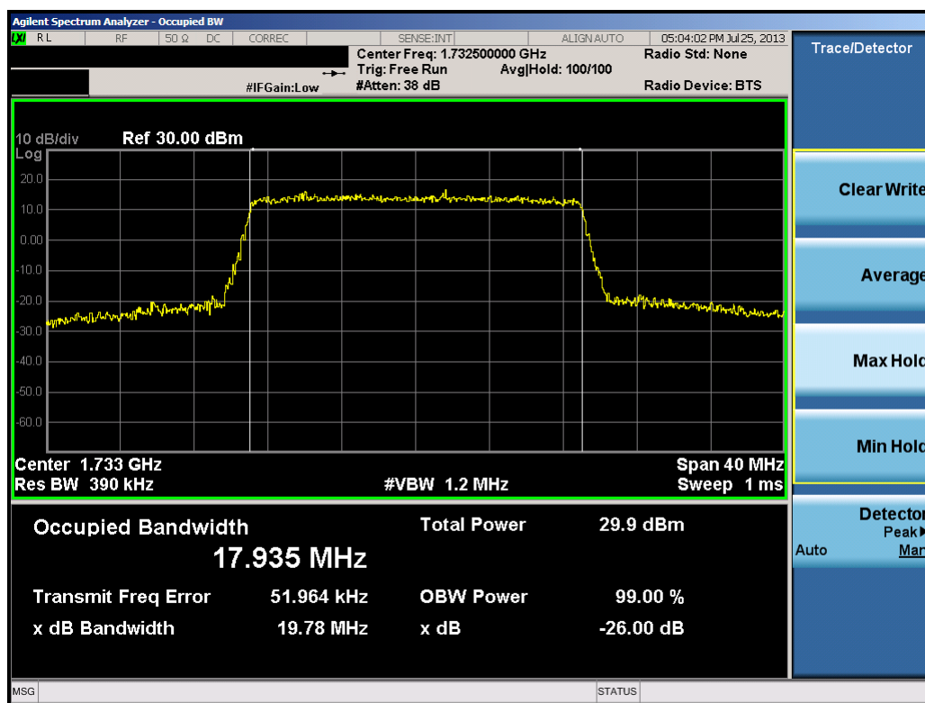
Plot 9-33. Occupied Bandwidth Plot (20.0MHz QPSK – RB Size 100)
