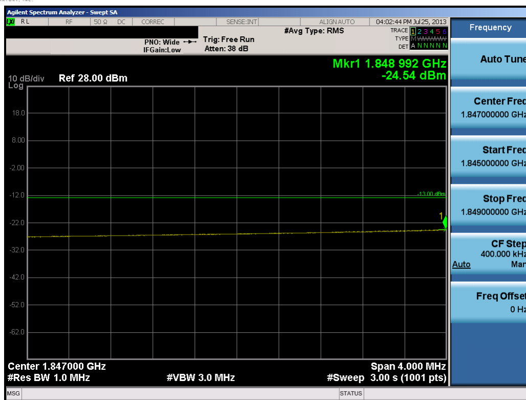
Plot 10-32. Lower Extended Band Edge Plot (20.0MHz QPSK – RB Size 100)
