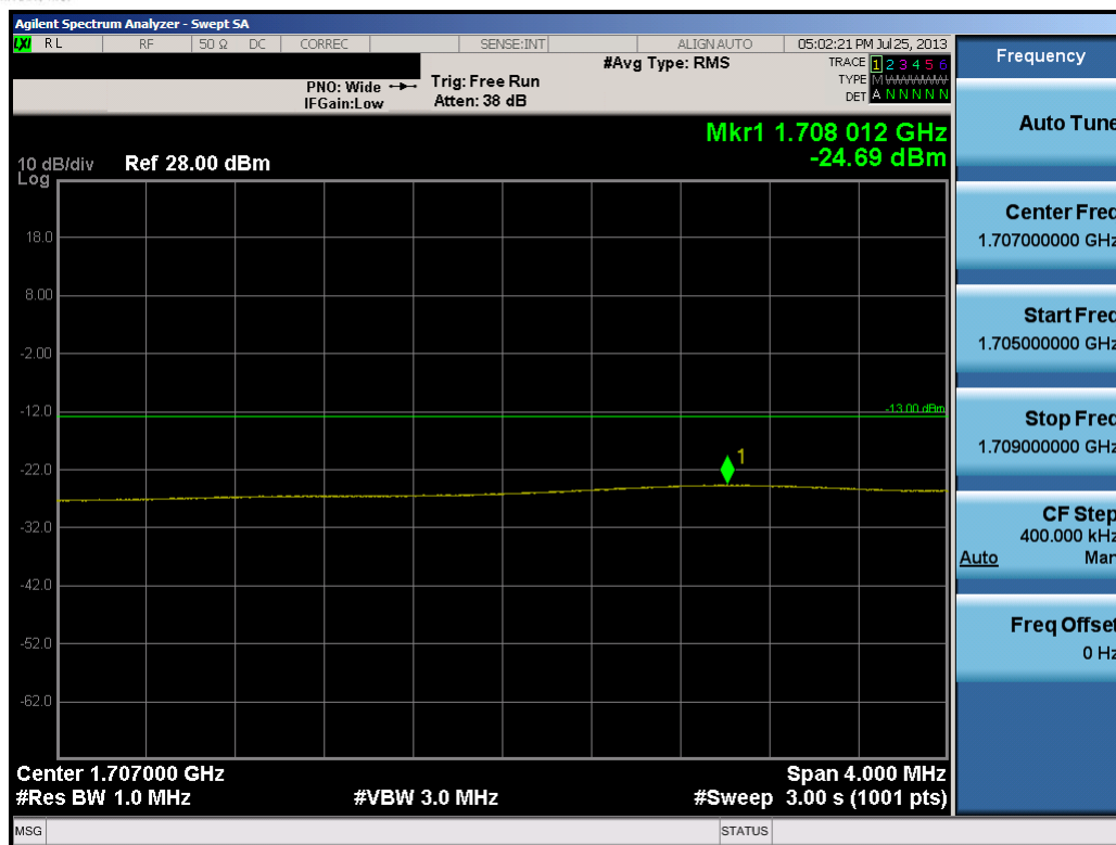
Plot 9-24. Lower Extended Band Edge Plot (15.0MHz QPSK – RB Size 75)
