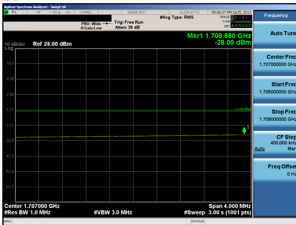
Plot 9-32. Lower Extended Band Edge Plot (20.0MHz QPSK – RB Size 100)
