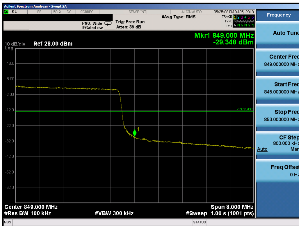
Plot 8-14. Upper Band Edge Plot (10.0MHz QPSK – RB Size 50)
